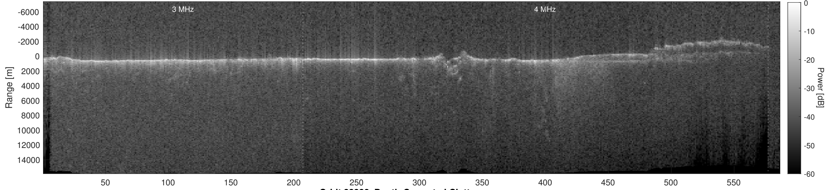
Orbit 22338, Depth-Corrected Cluttergram
