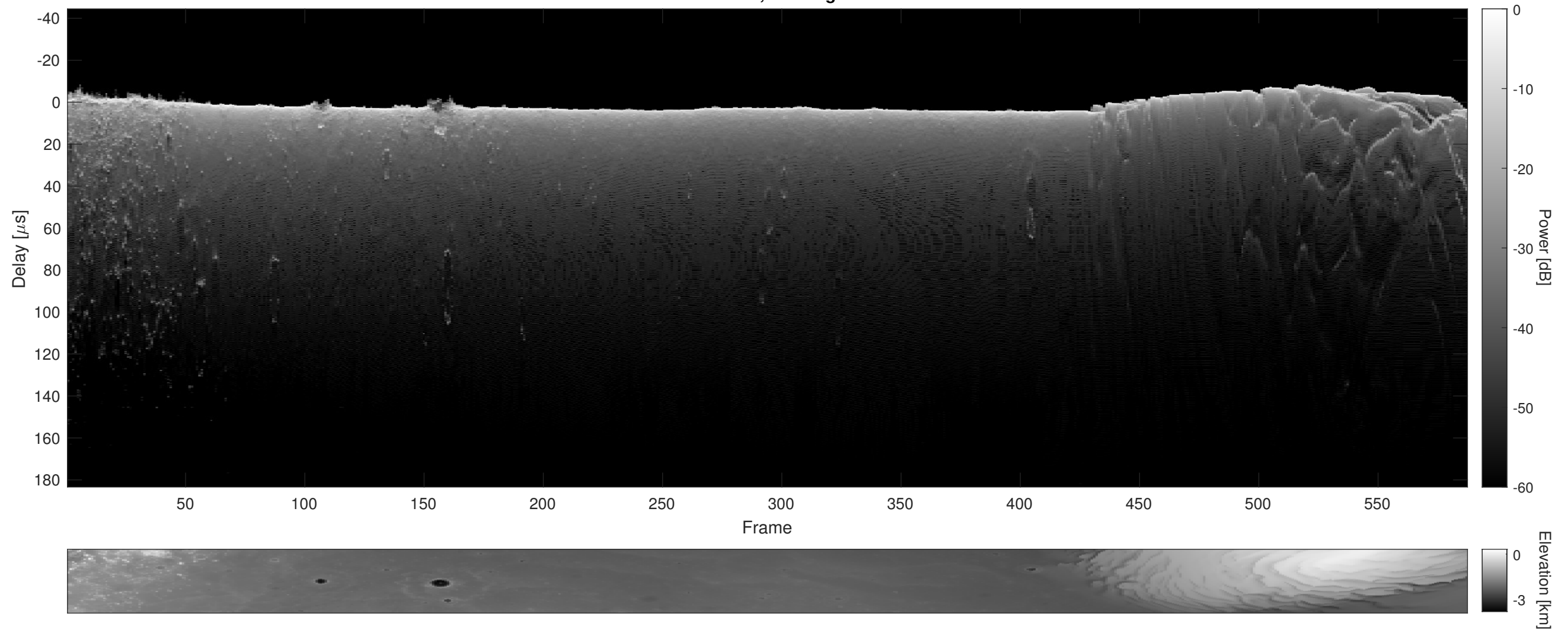
Orbit 22339, Cluttergram
