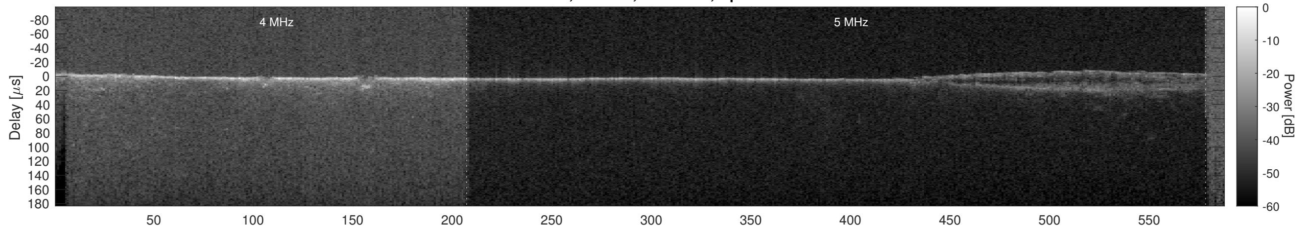
Orbit 22339, Cluttergram
