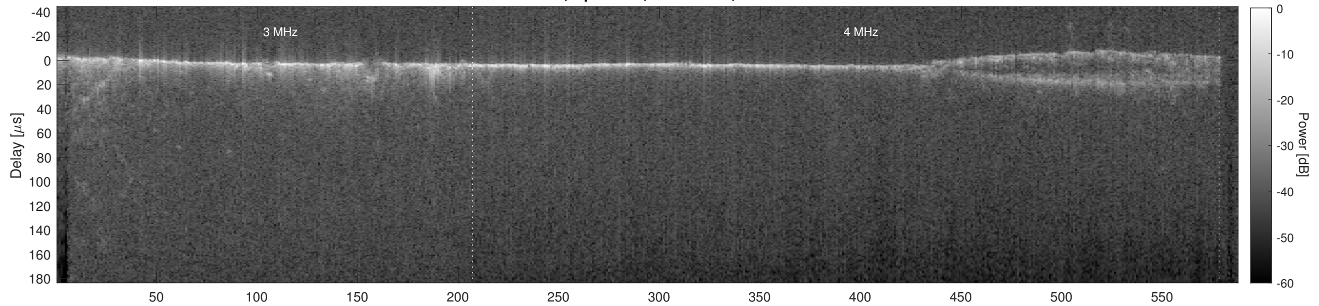
Orbit 22339, Cluttergram
