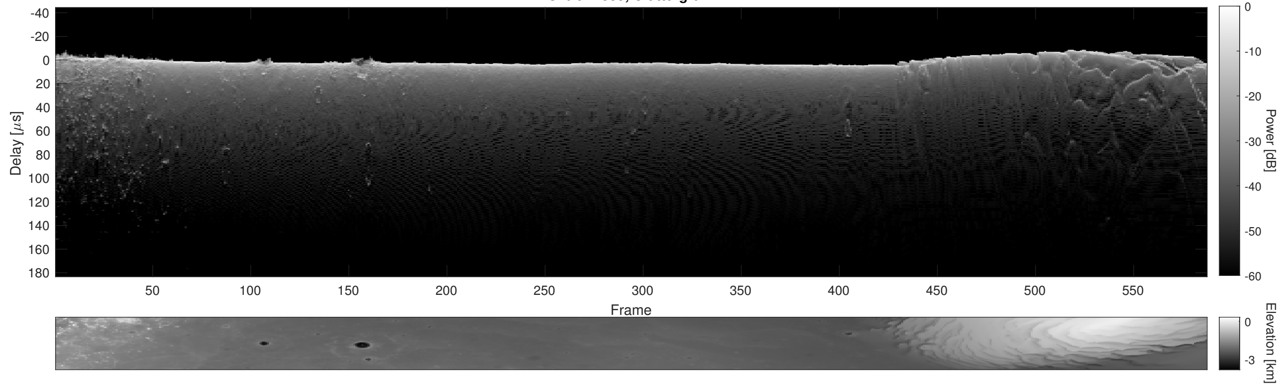
Orbit 22339, Cluttergram
