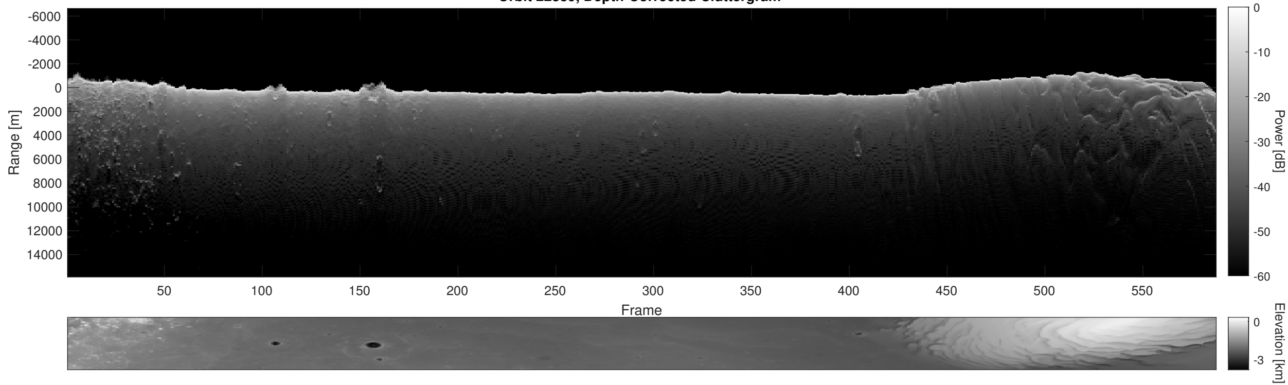
Orbit 22339, Depth-Corrected Cluttergram
