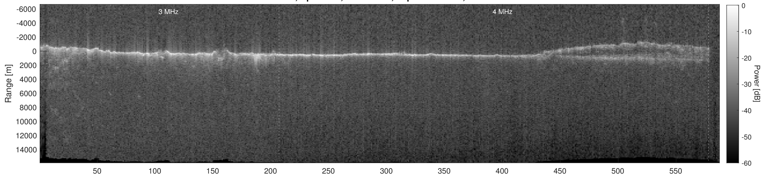
Orbit 22339, Depth-Corrected Cluttergram
