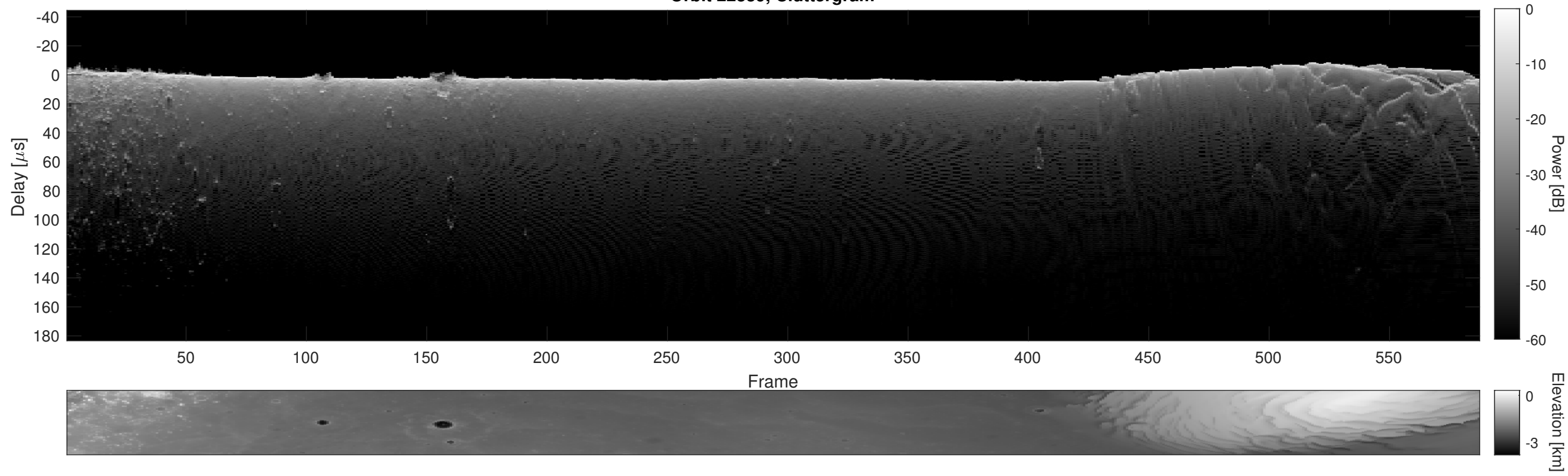
Orbit 22339, Cluttergram
