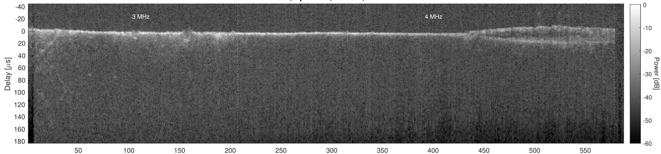
Orbit 22339, Cluttergram
