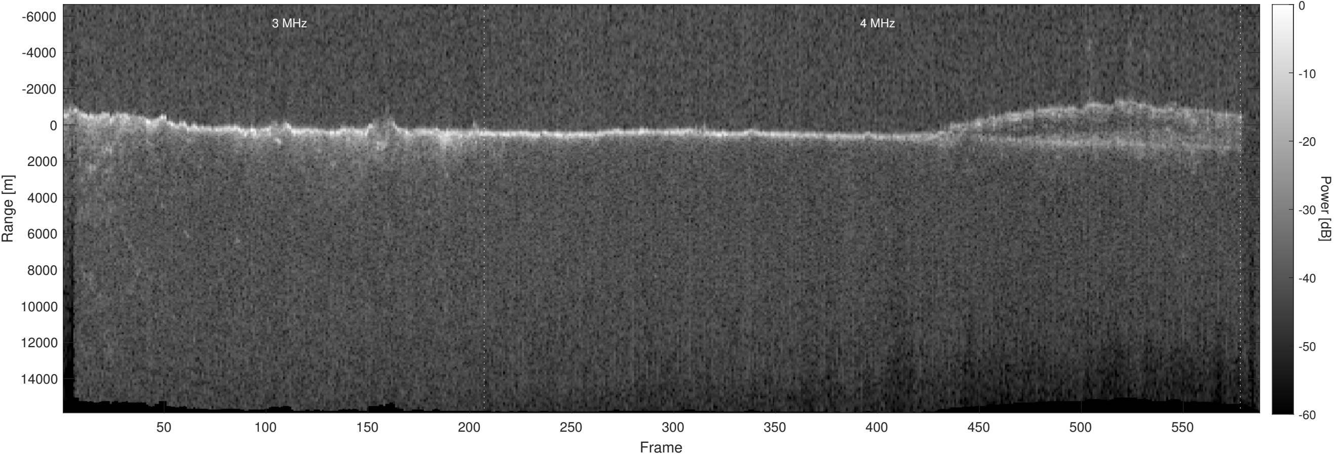
Orbit 22339, Optimized, Window, Depth-Corrected, Channel 2
