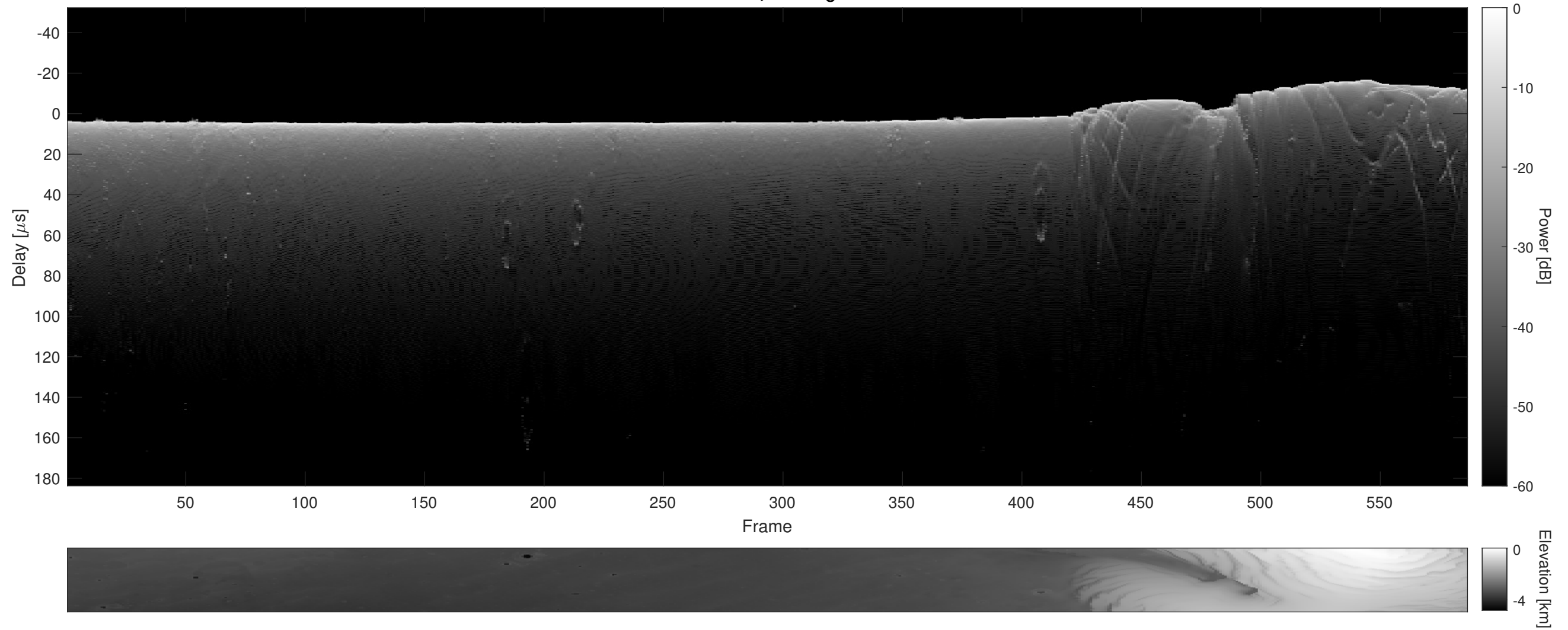
Orbit 22340, Cluttergram
