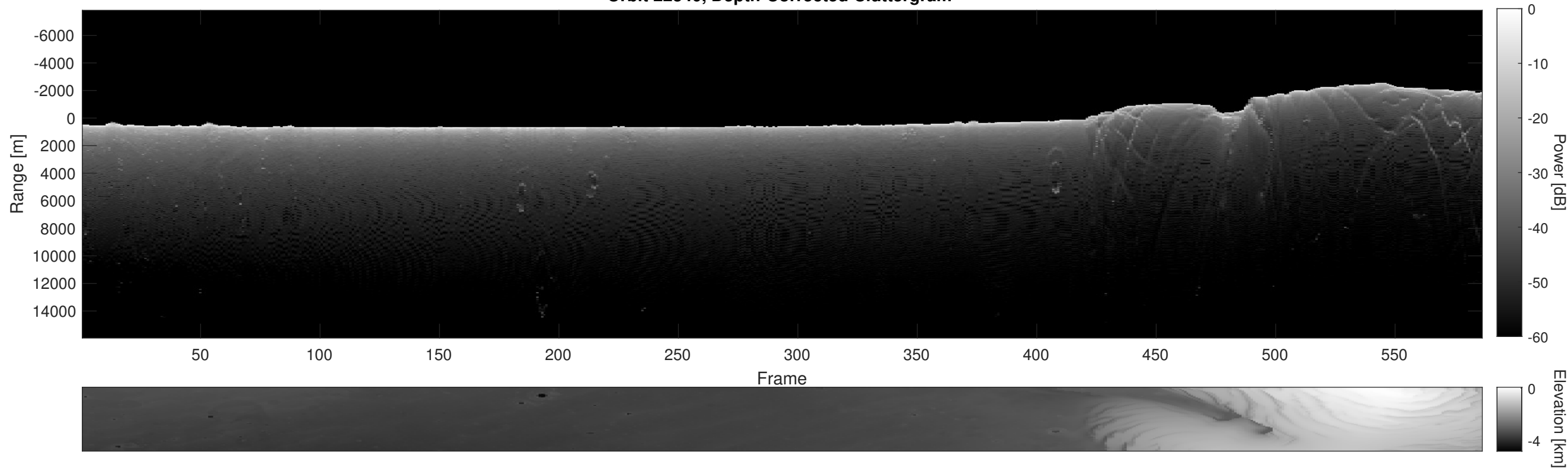
Orbit 22340, Depth-Corrected Cluttergram
