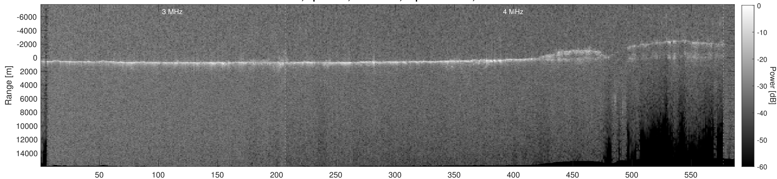
Orbit 22340, Depth-Corrected Cluttergram
