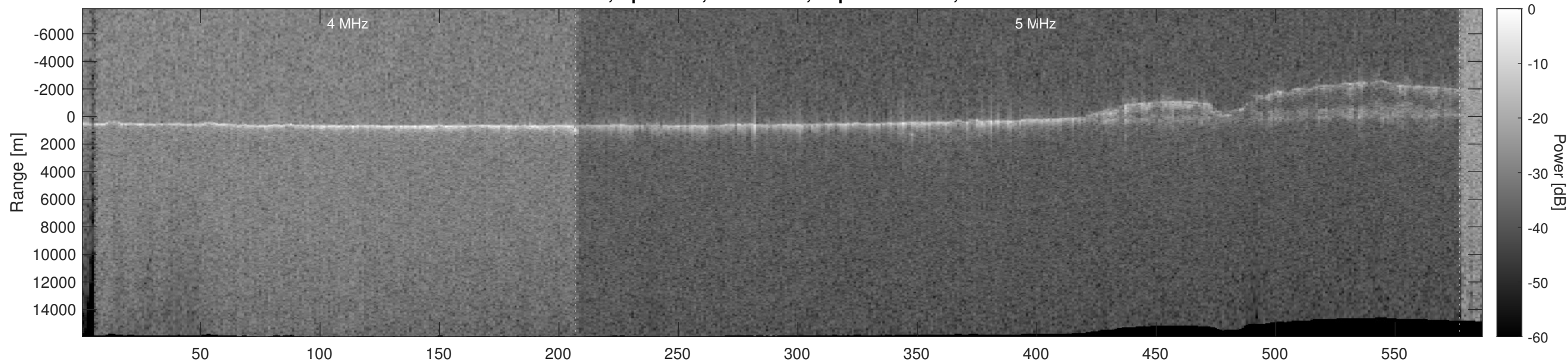
Orbit 22340, Optimized, No Window, Depth-Corrected, Channel 2
