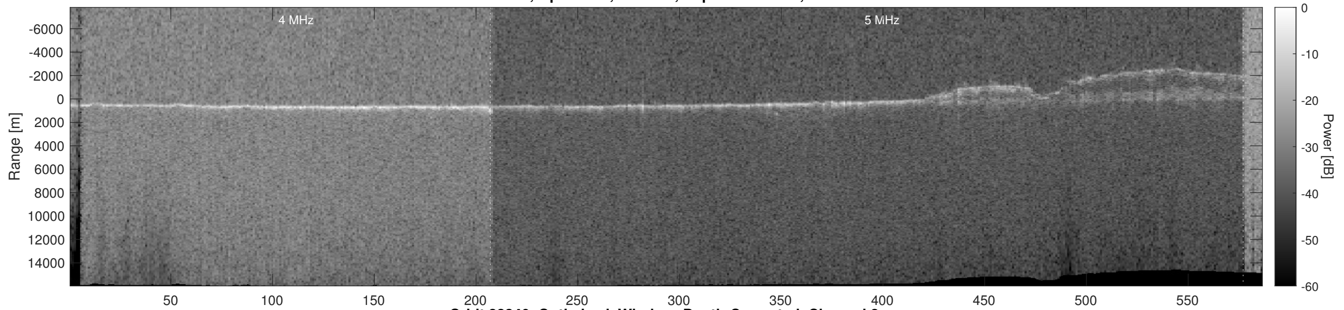
Orbit 22340, Optimized, Window, Depth-Corrected, Channel 2
