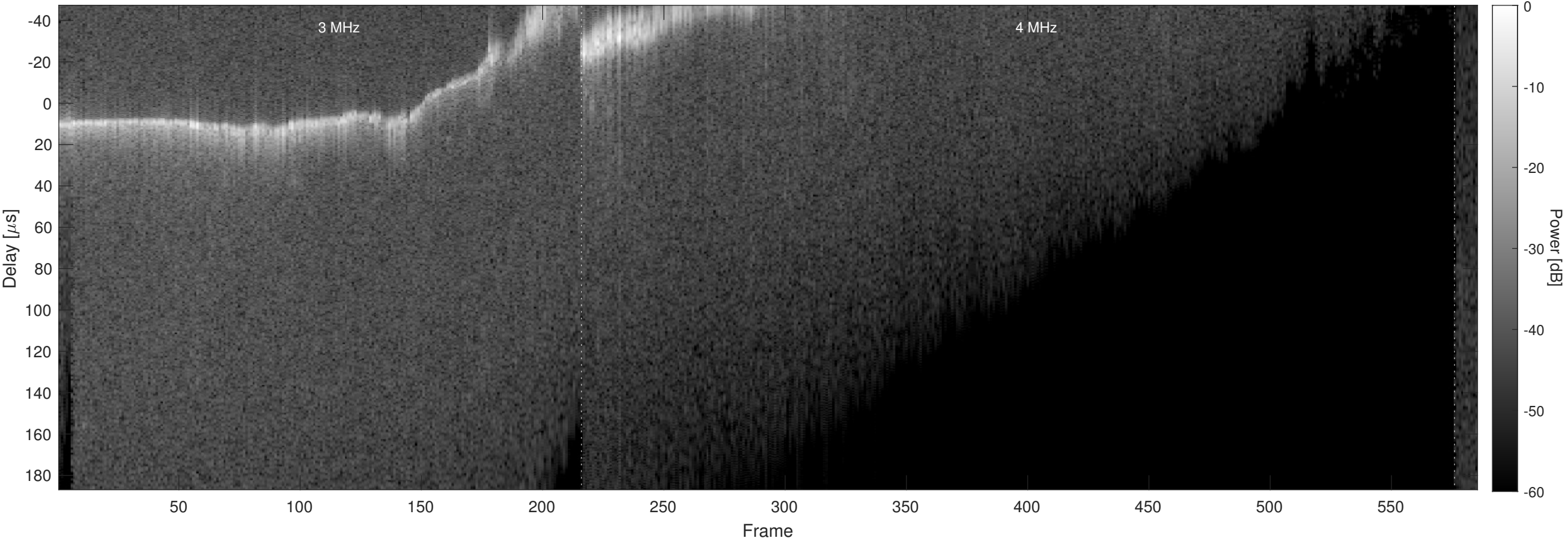
Orbit 22342, Chapman, No Window, Channel 2
