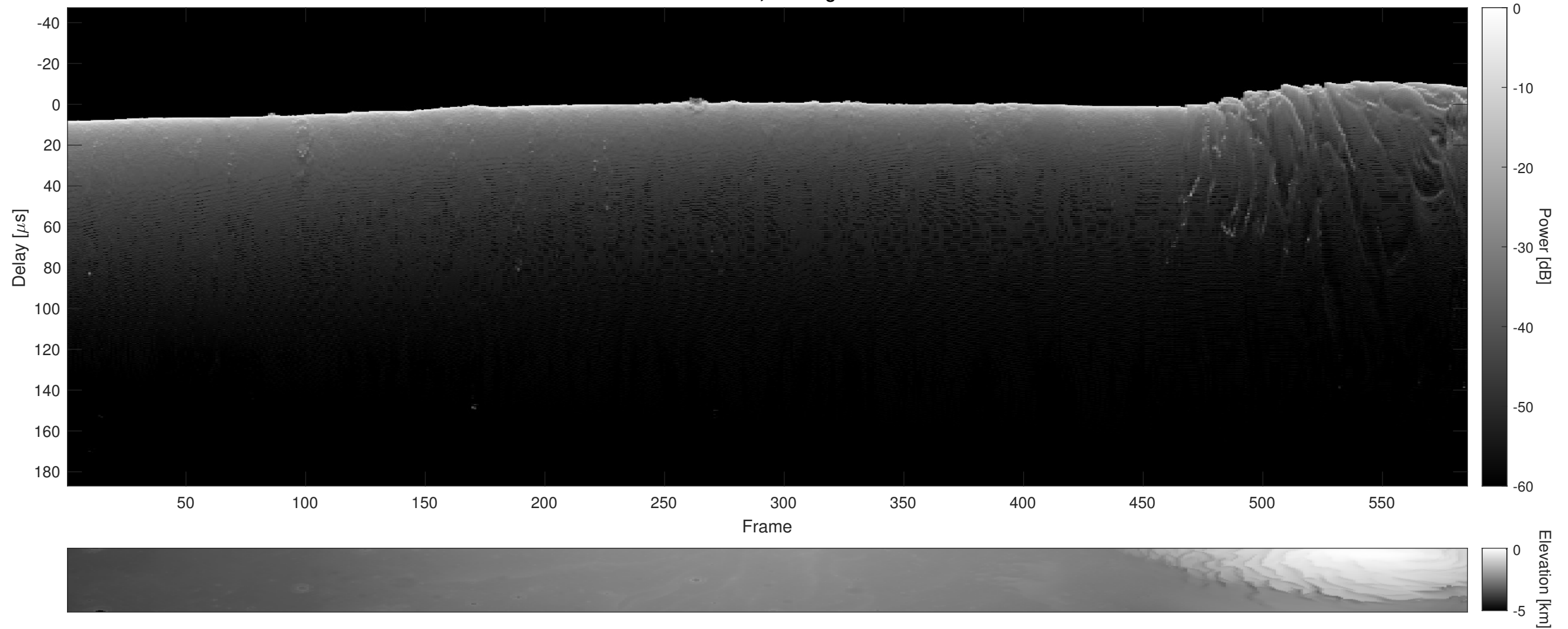
Orbit 22342, Cluttergram
