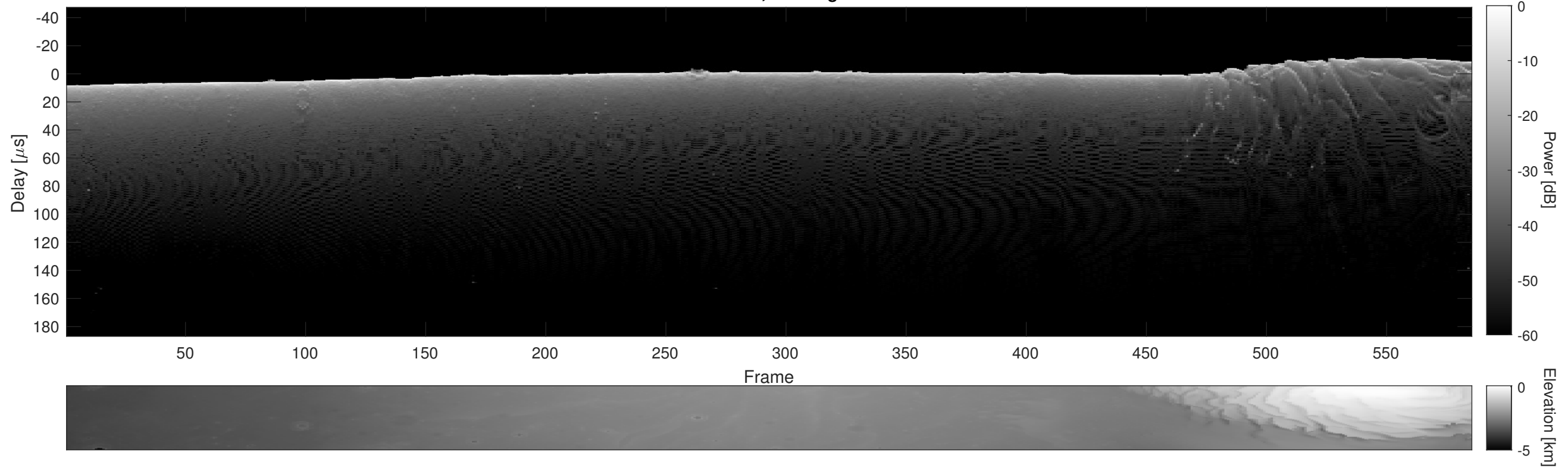
Orbit 22342, Cluttergram
