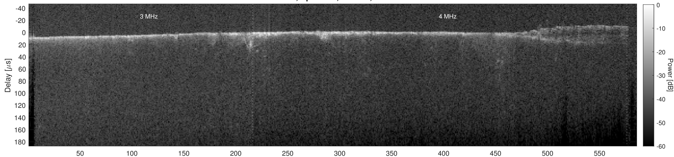
Orbit 22342, Cluttergram
