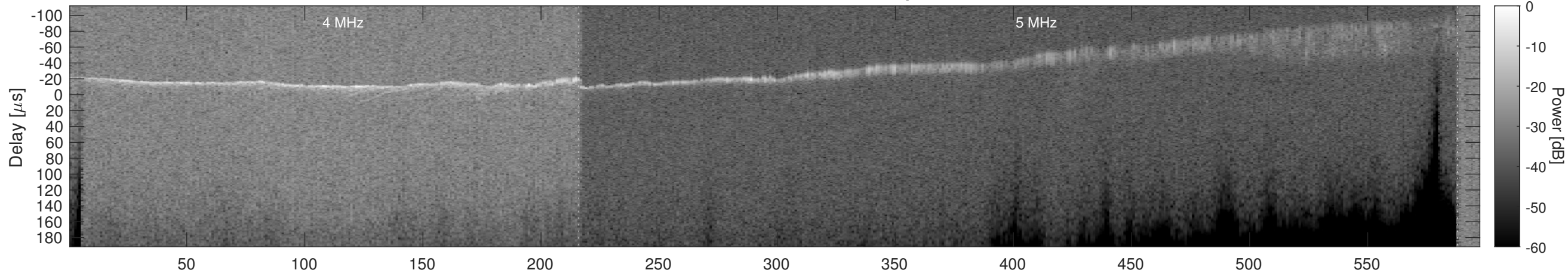
Orbit 22344, Window, Channel 1, Optimized
