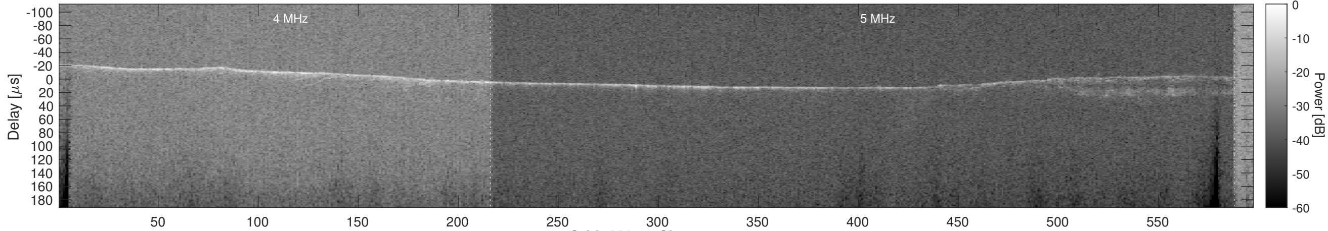
Orbit 22344, Cluttergram
