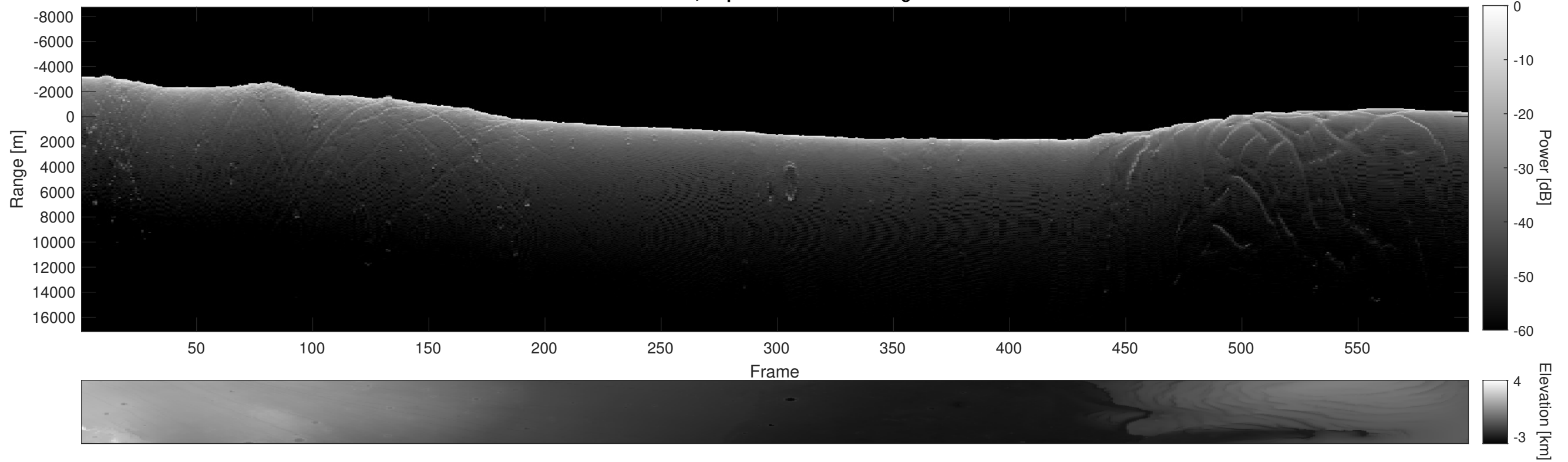
Orbit 22344, Depth-Corrected Cluttergram
