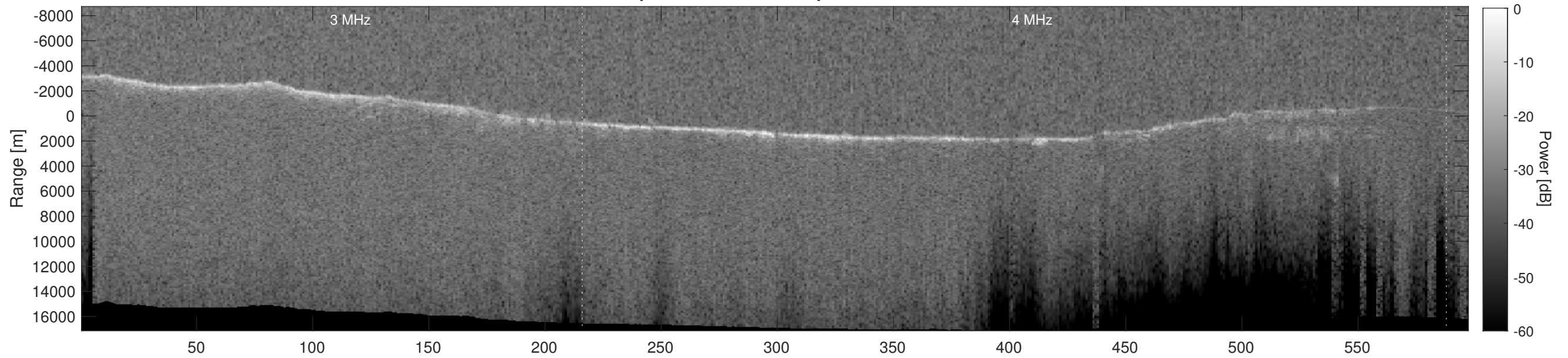
Orbit 22344, Depth-Corrected Cluttergram
