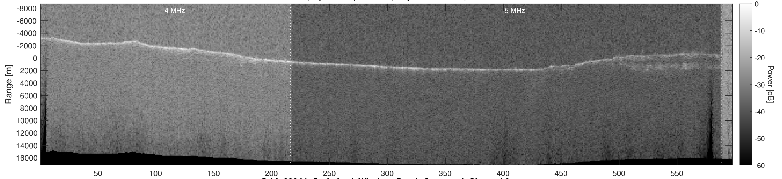
Orbit 22344, Optimized, Window, Depth-Corrected, Channel 2
