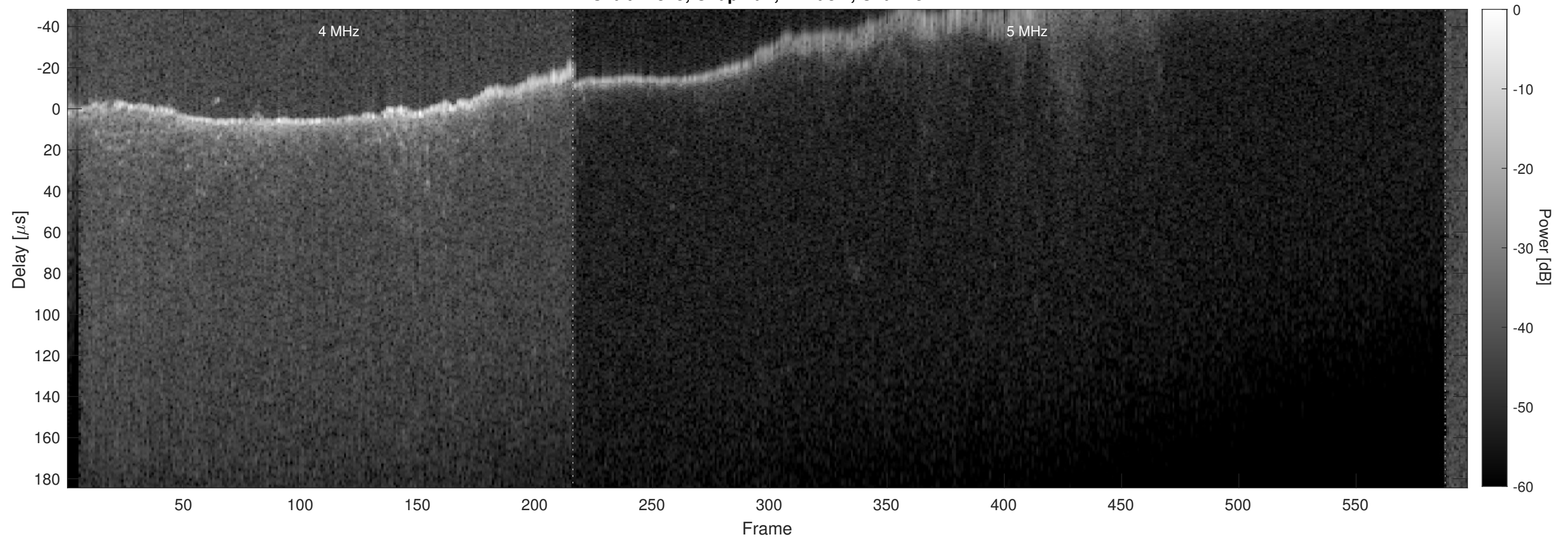
Orbit 22345, Chapman, Window, Channel 2
