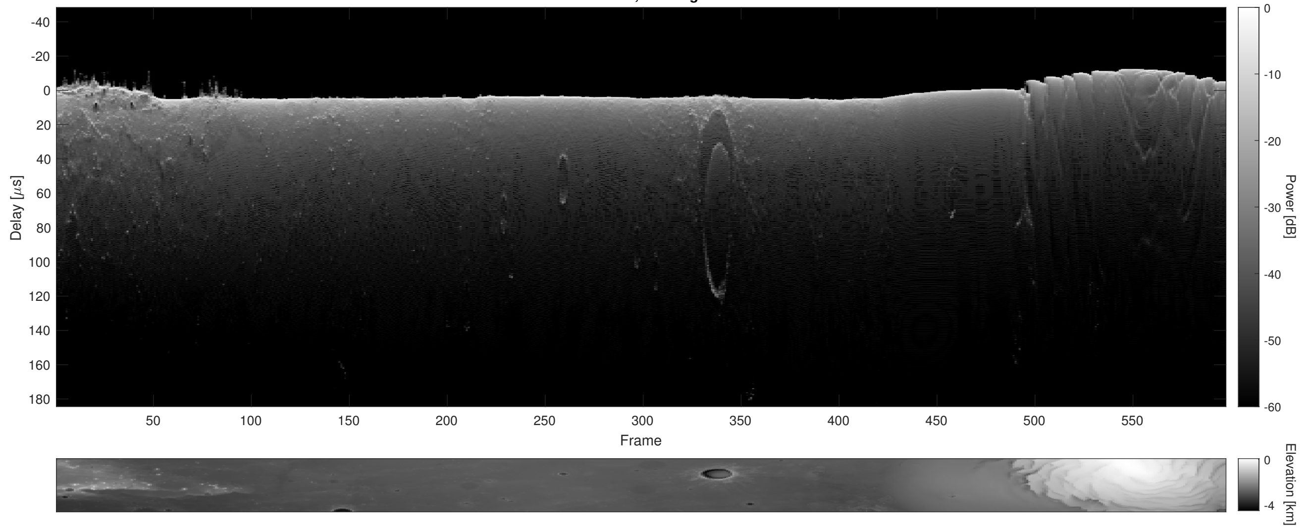
Orbit 22345, Cluttergram
