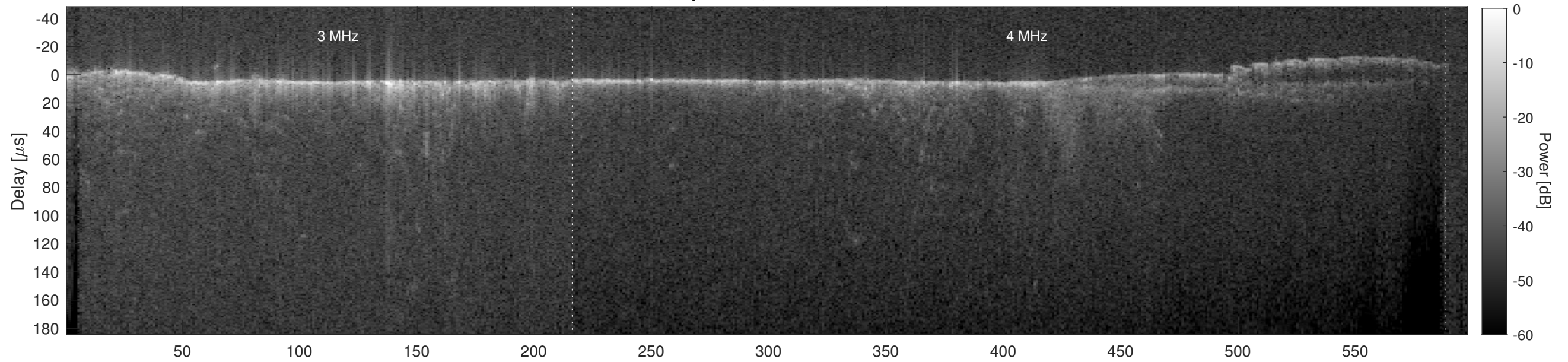
Orbit 22345, Cluttergram
