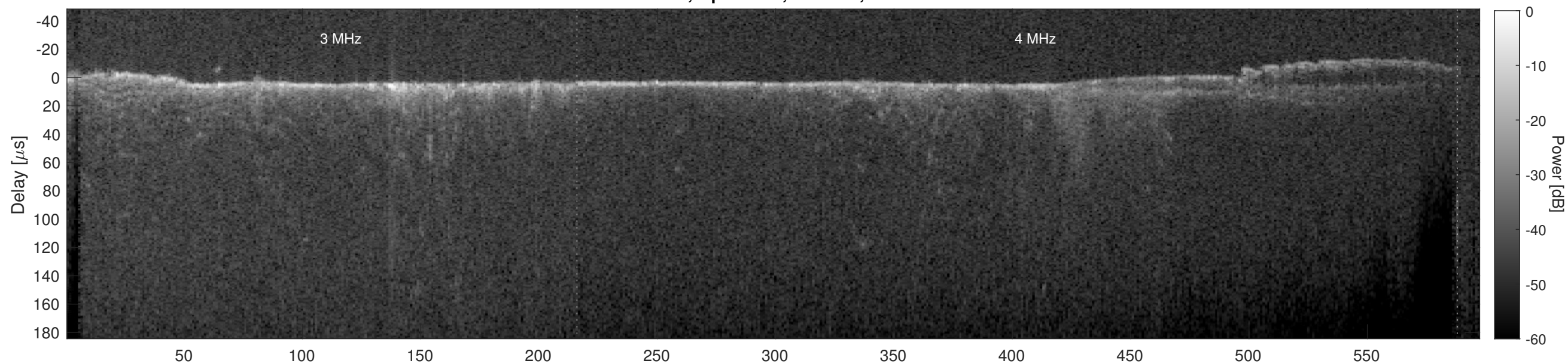
Orbit 22345, Cluttergram
