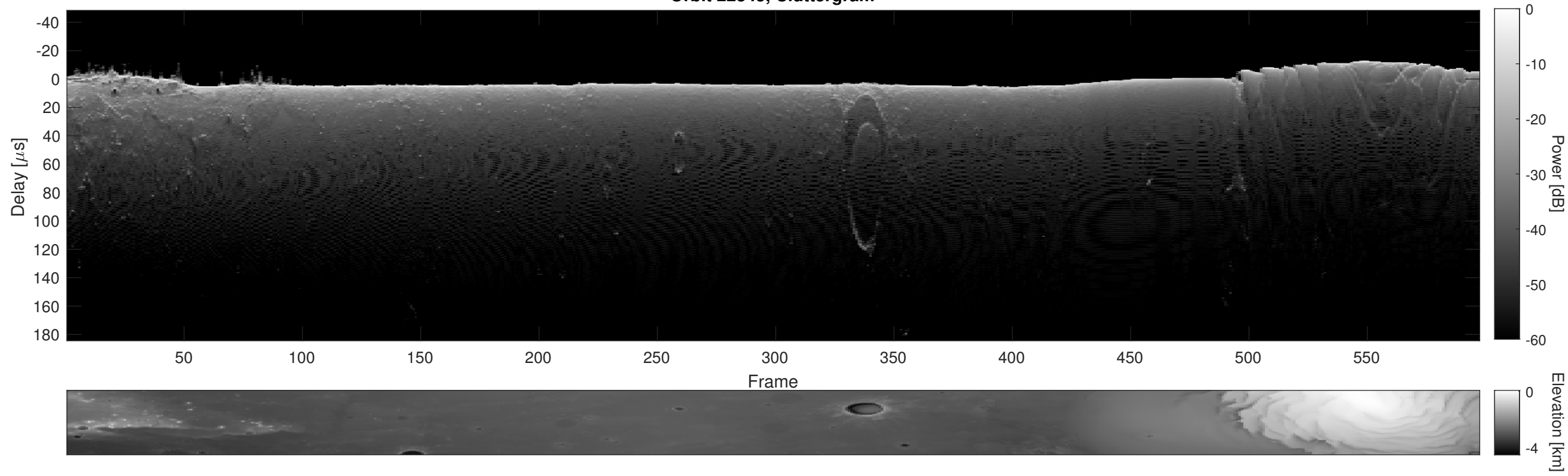
Orbit 22345, Cluttergram
