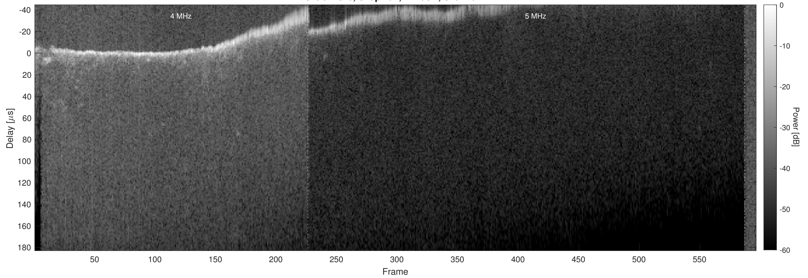
Orbit 22346, Chapman, Window, Channel 2
