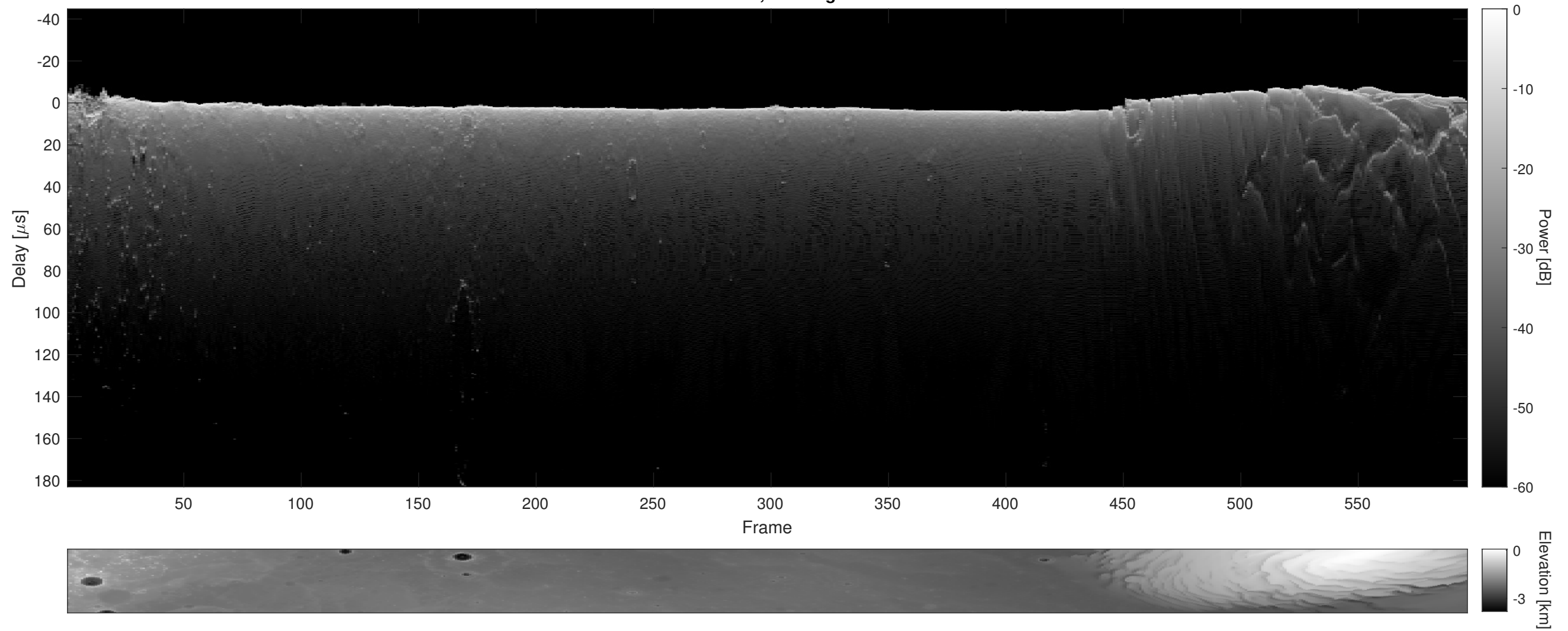
Orbit 22346, Cluttergram
