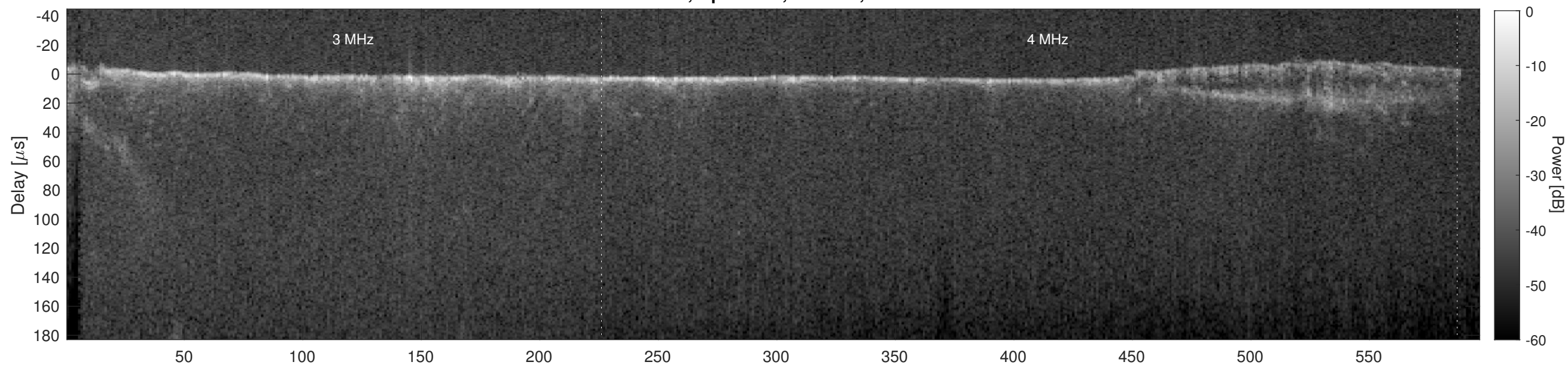
Orbit 22346, Cluttergram
