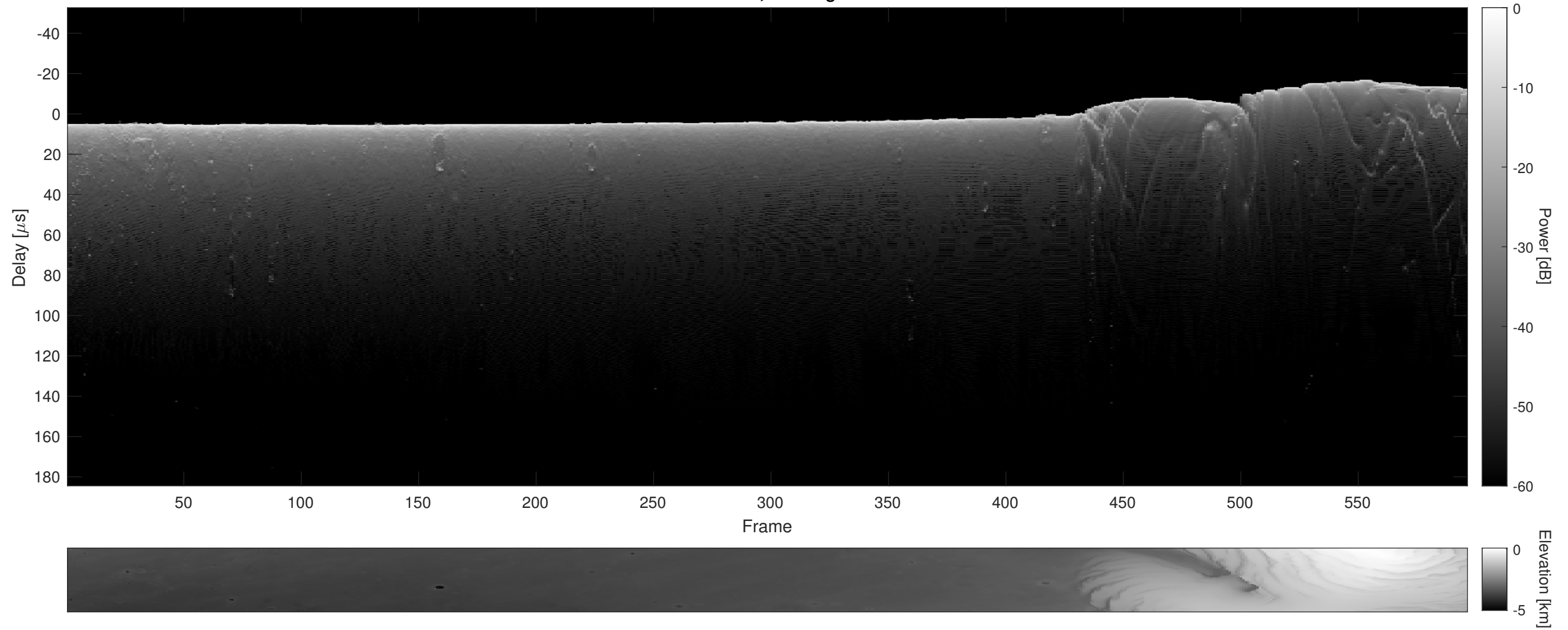
Orbit 22347, Cluttergram
