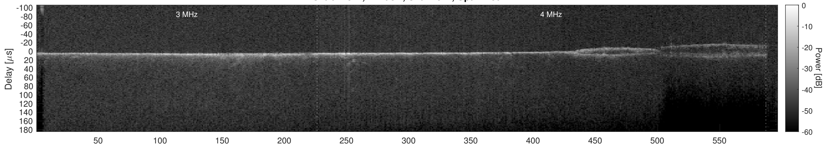
Orbit 22347, Cluttergram
