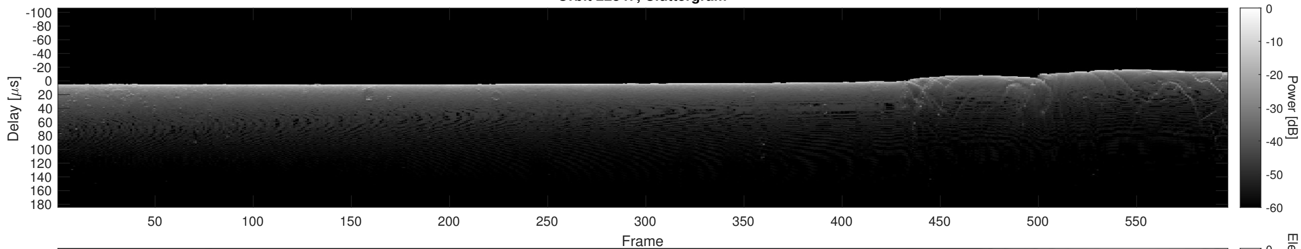
Orbit 22347, Cluttergram
