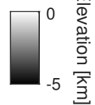
Elevation [km]
