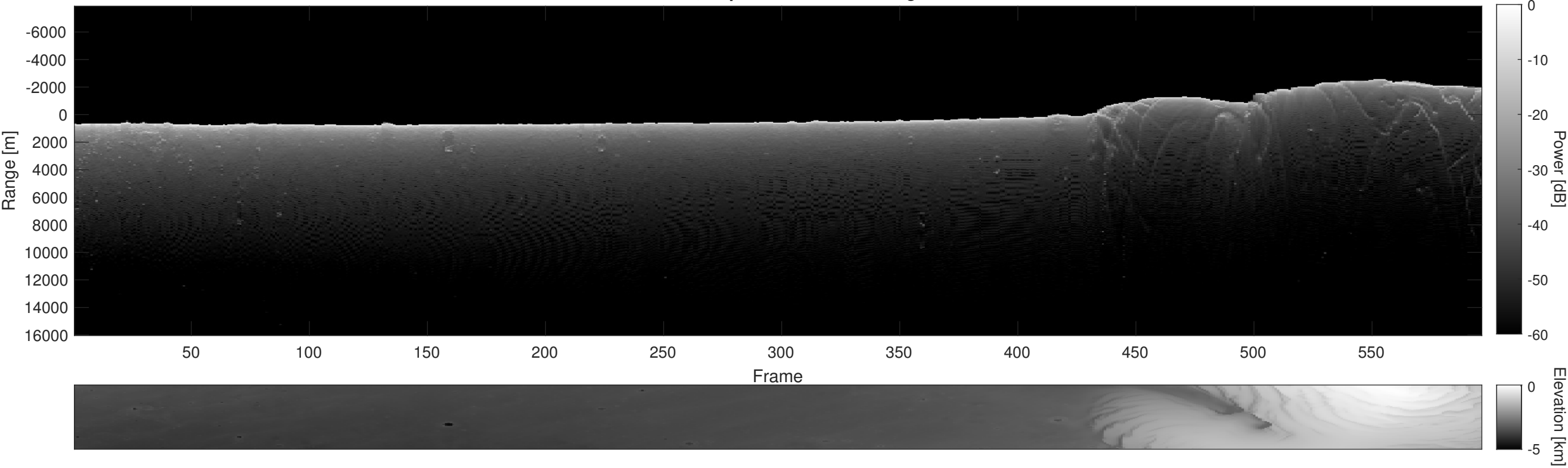
Orbit 22347, Depth-Corrected Cluttergram
