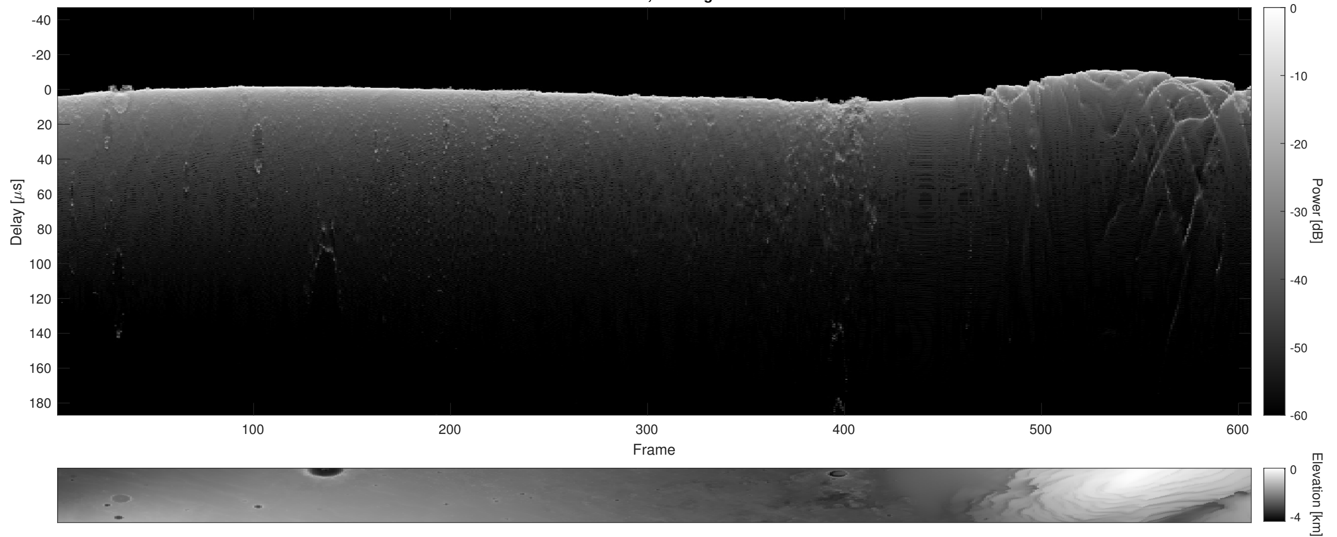
Orbit 22348, Cluttergram
