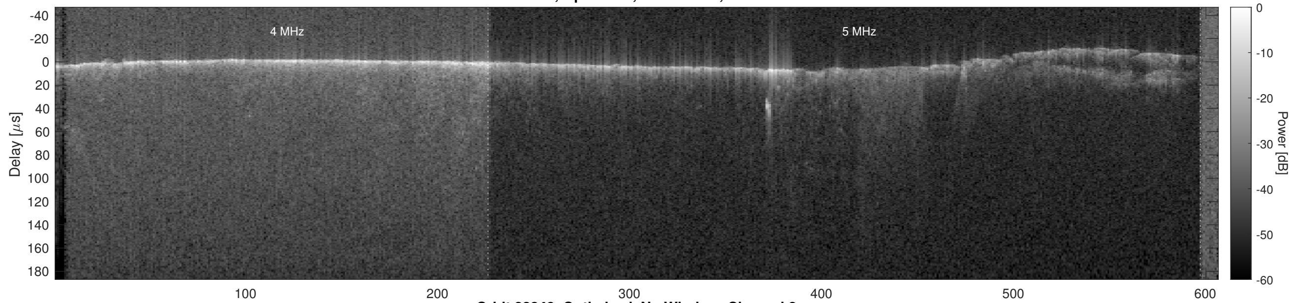
Orbit 22348, Optimized, No Window, Channel 2
