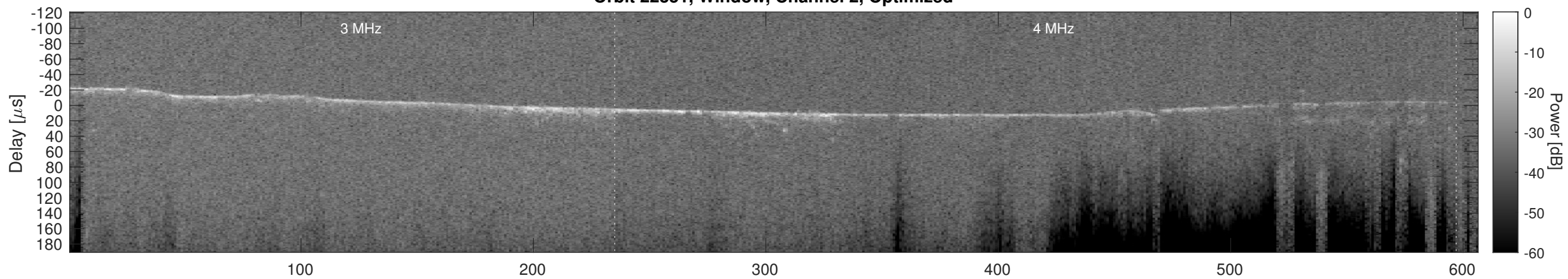
Orbit 22351, Cluttergram
