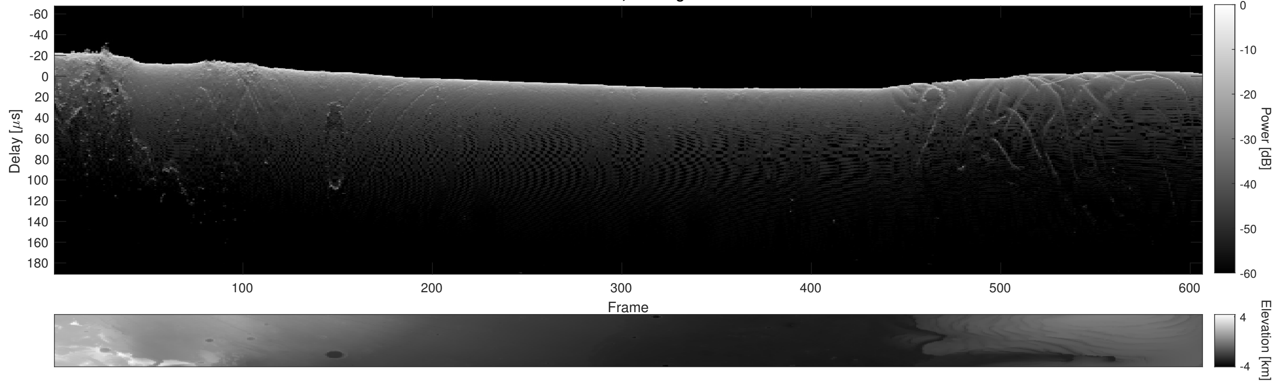
Orbit 22351, Cluttergram
