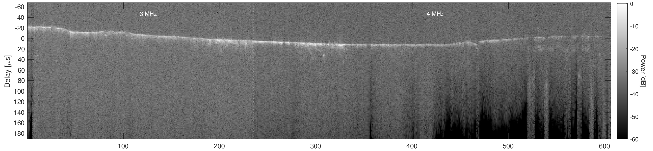
Orbit 22351, Cluttergram
