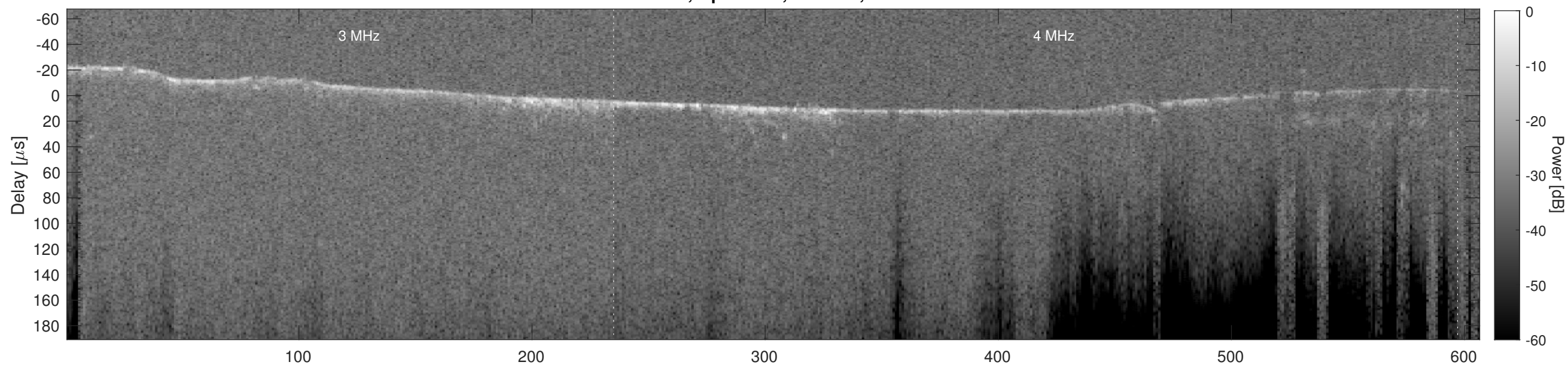
Orbit 22351, Cluttergram
