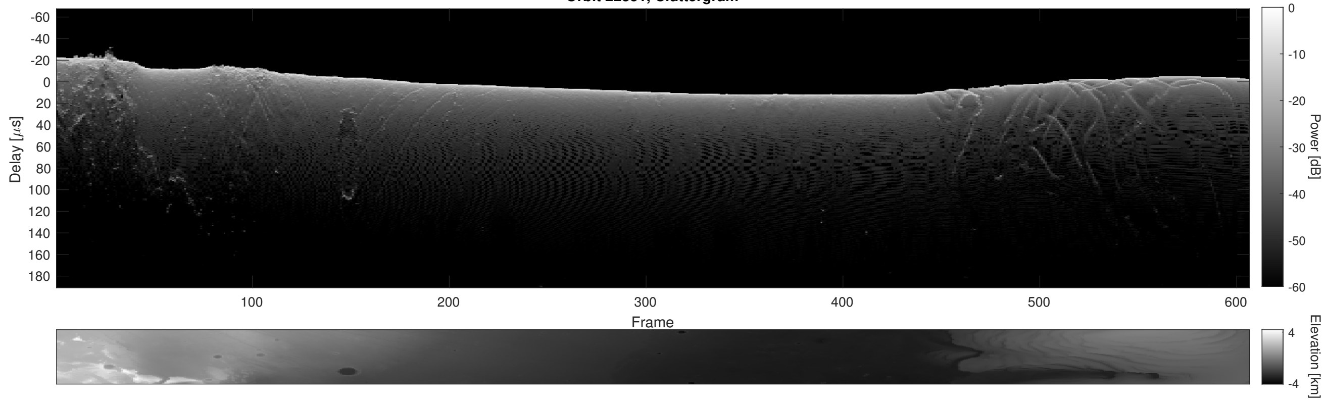
Orbit 22351, Cluttergram
