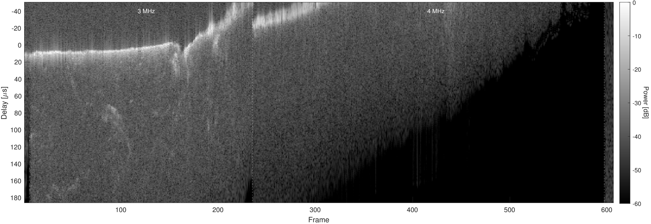
Orbit 22352, Chapman, No Window, Channel 2
