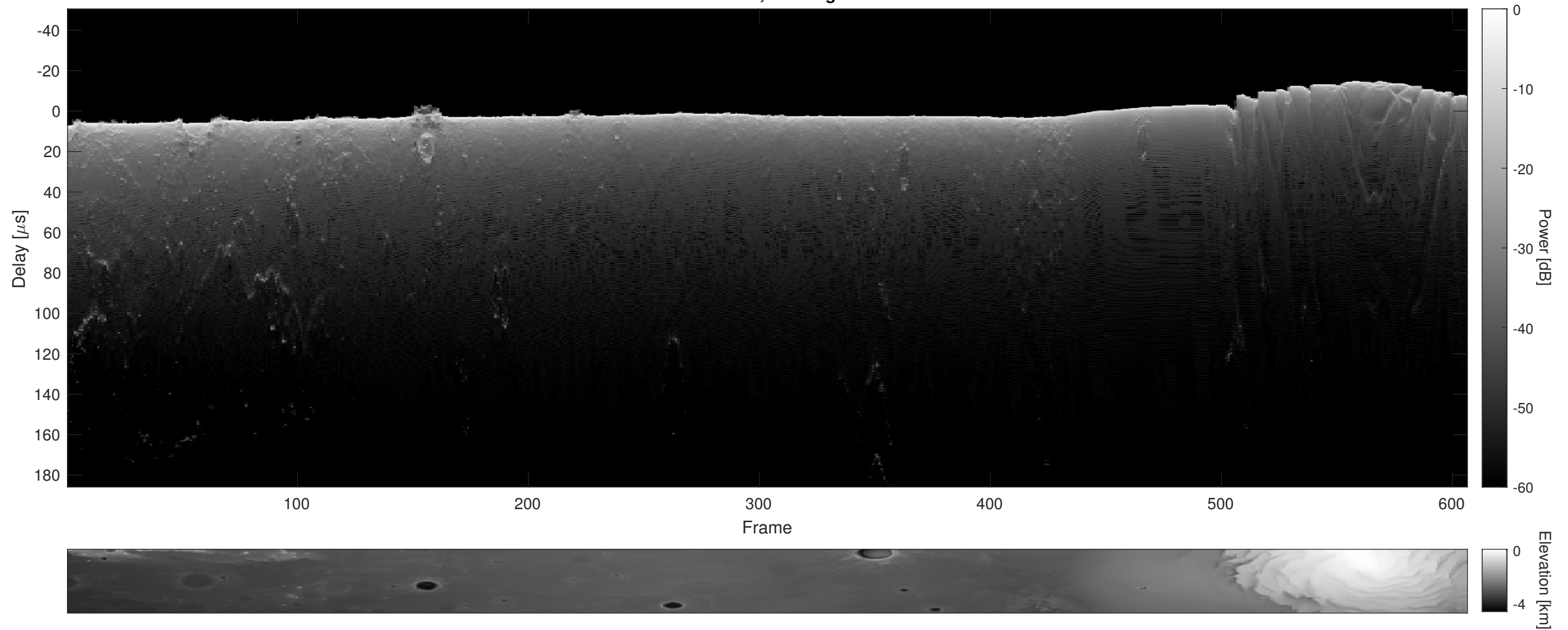
Orbit 22352, Cluttergram
