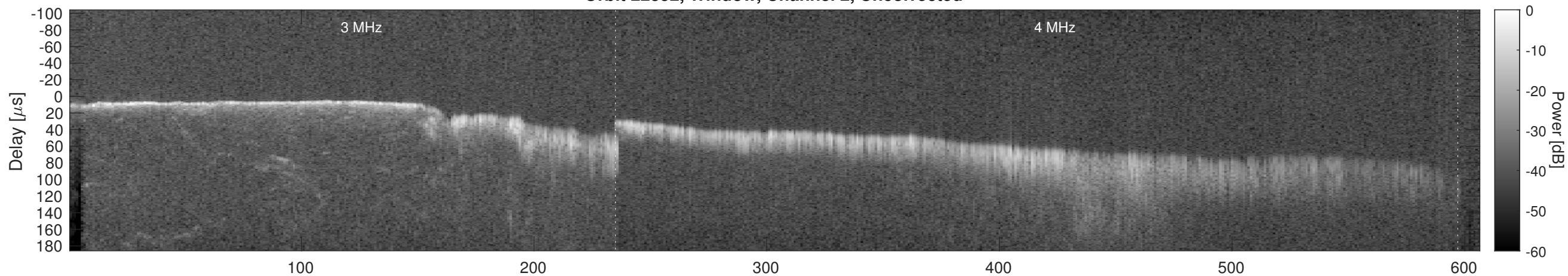
Orbit 22352, Window, Channel 2, Chapman
