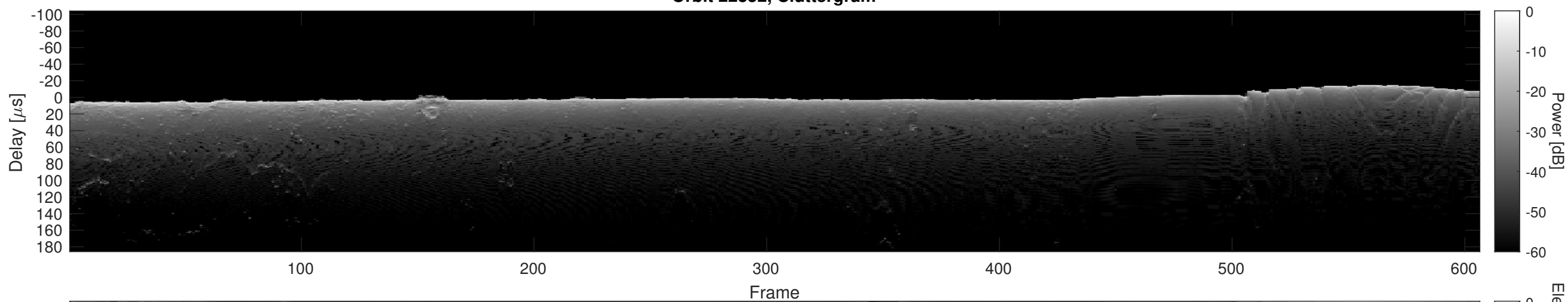
Orbit 22352, Cluttergram
