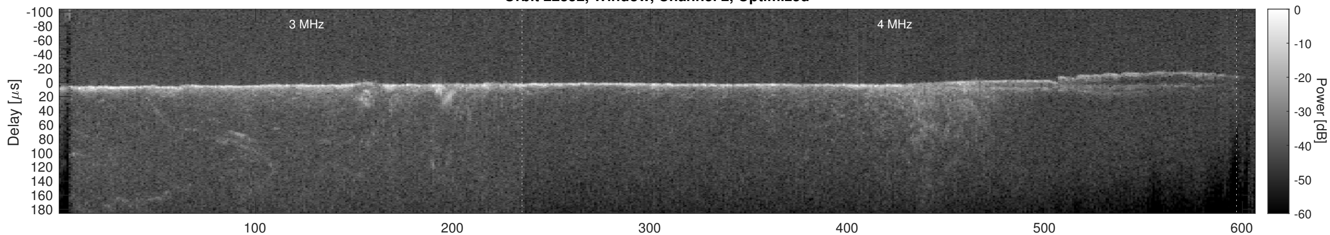
Orbit 22352, Cluttergram
