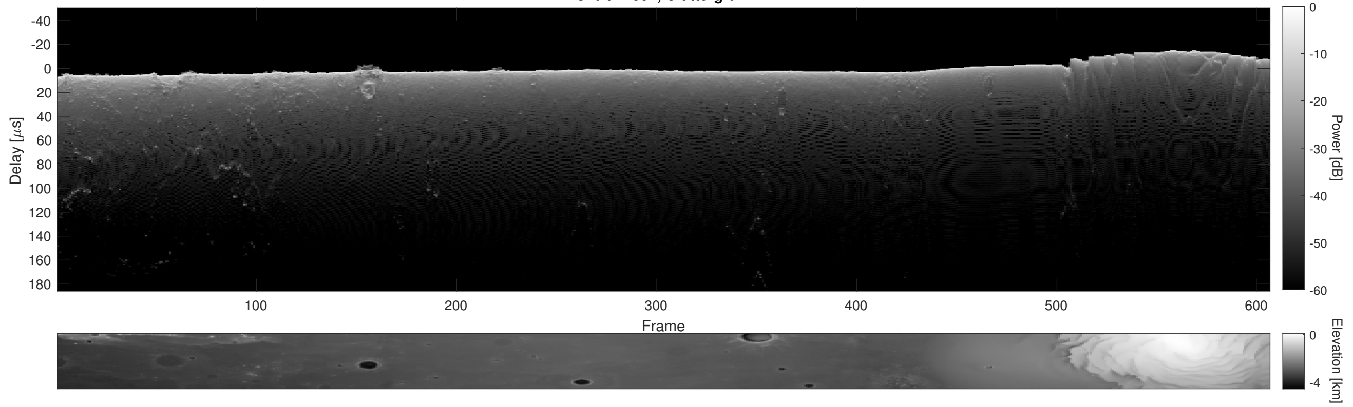
Orbit 22352, Cluttergram
