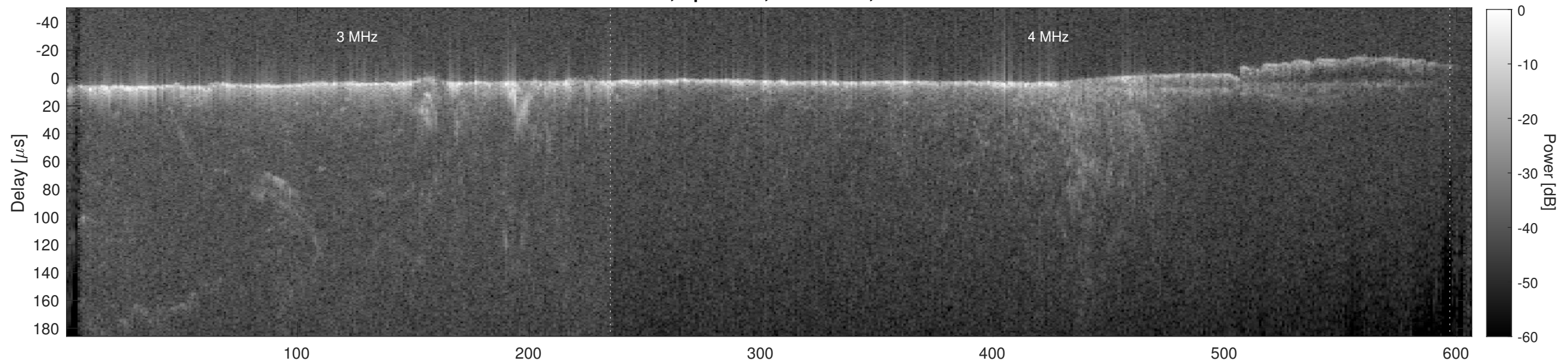
Orbit 22352, Cluttergram
