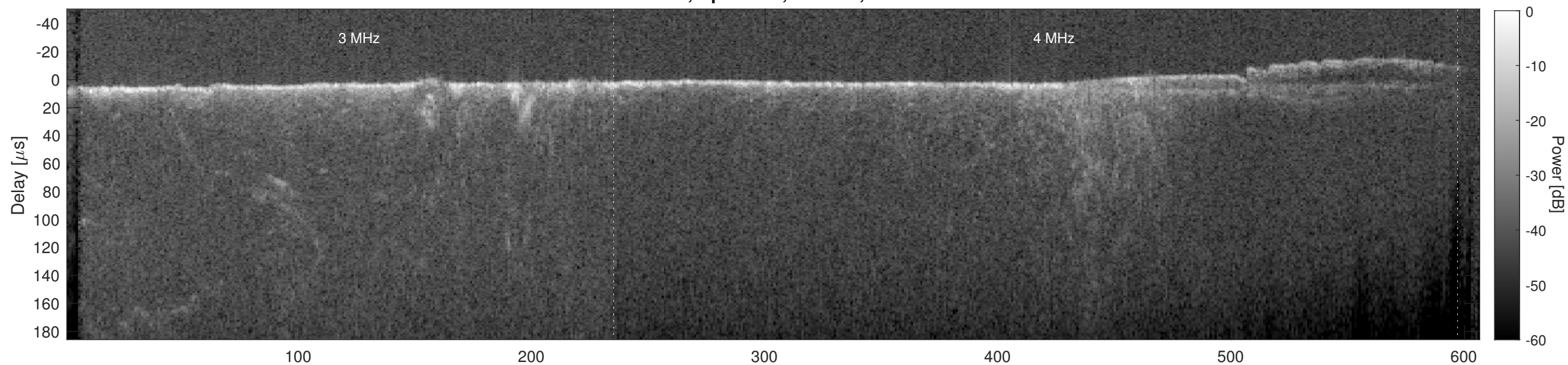
Orbit 22352, Cluttergram
