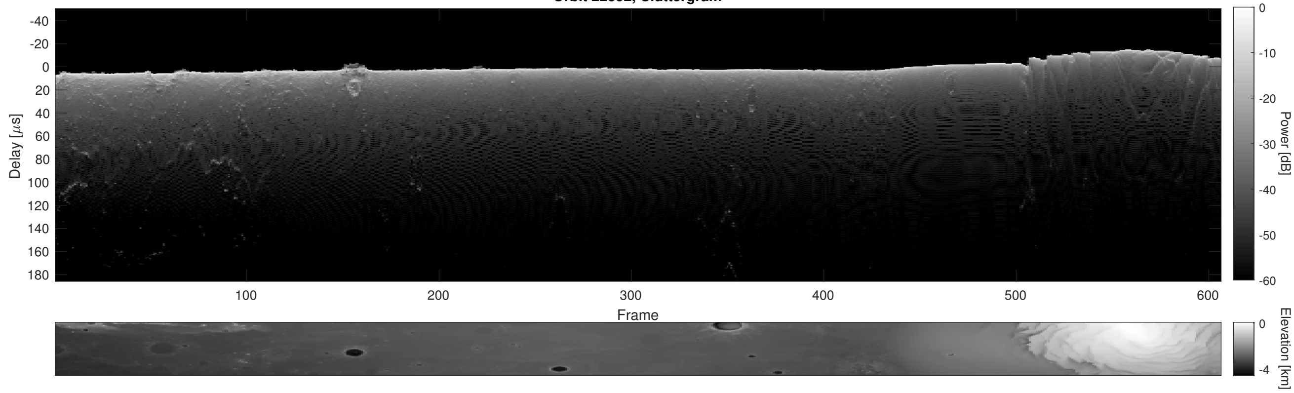
Orbit 22352, Cluttergram
