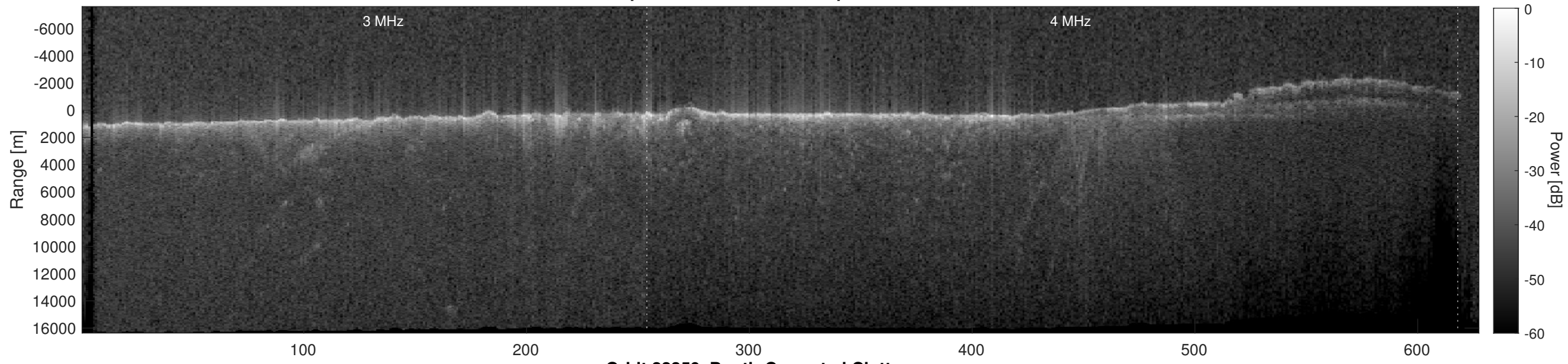
Orbit 22359, Depth-Corrected Cluttergram
