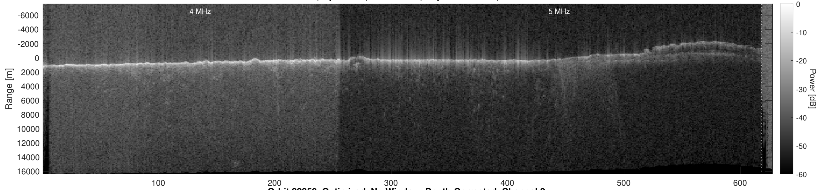
Orbit 22359, Optimized, No Window, Depth-Corrected, Channel 2
