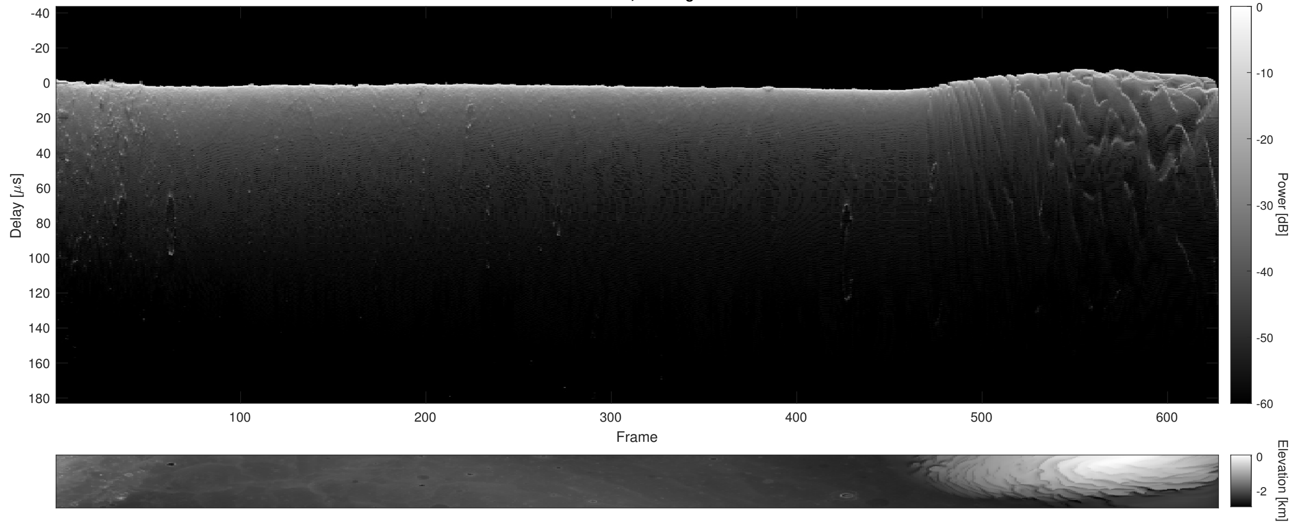
Orbit 22360, Cluttergram
