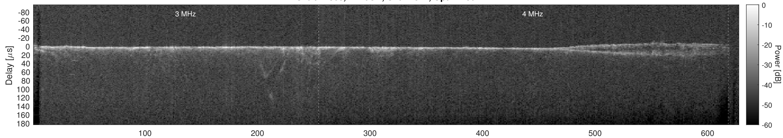
Orbit 22360, Cluttergram
