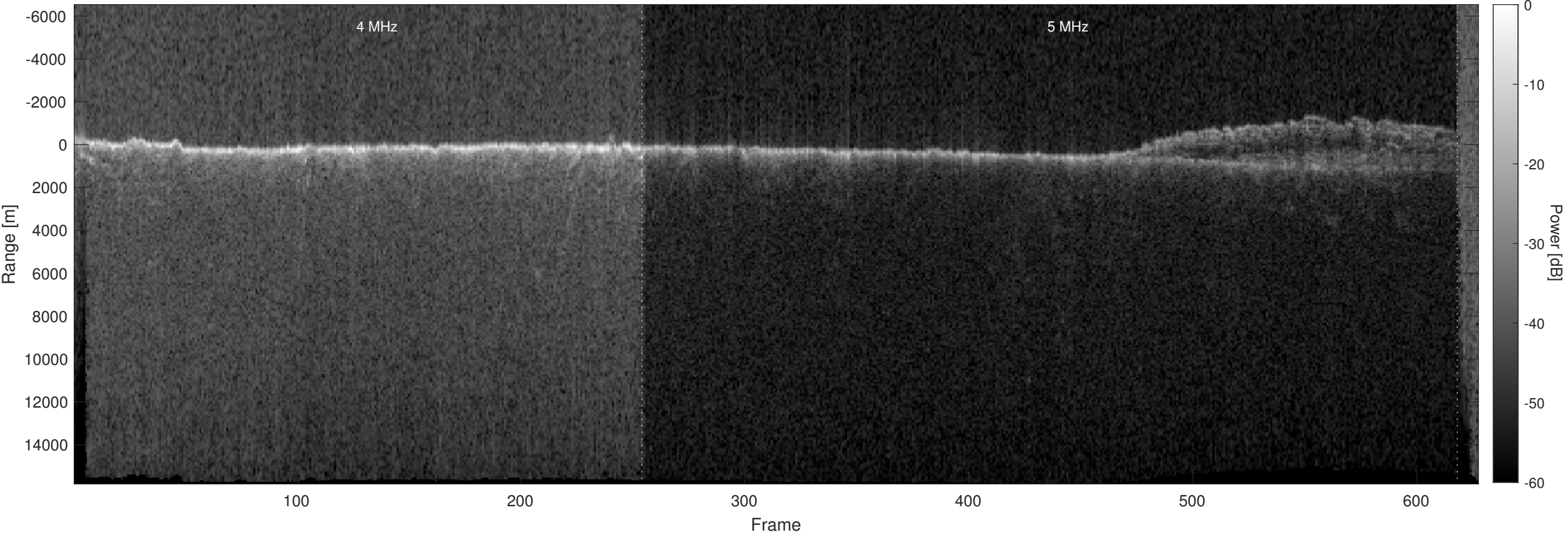
Orbit 22360, Optimized, Window, Depth-Corrected, Channel 2
