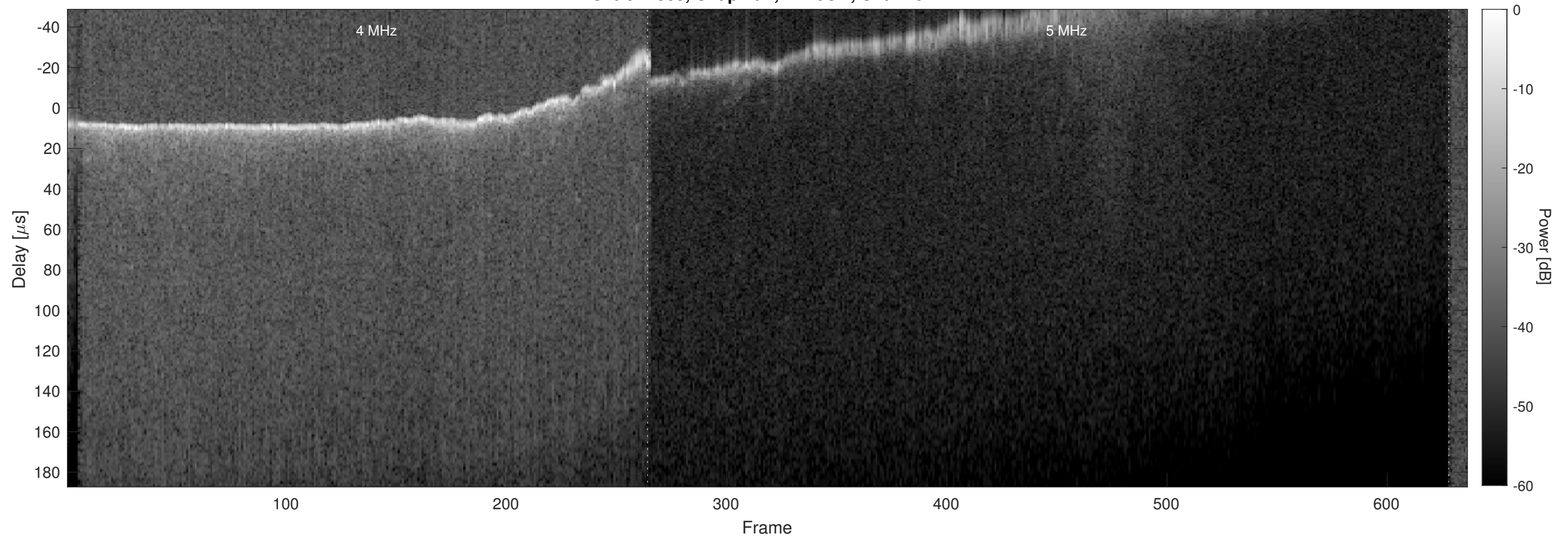
Orbit 22363, Chapman, Window, Channel 2
