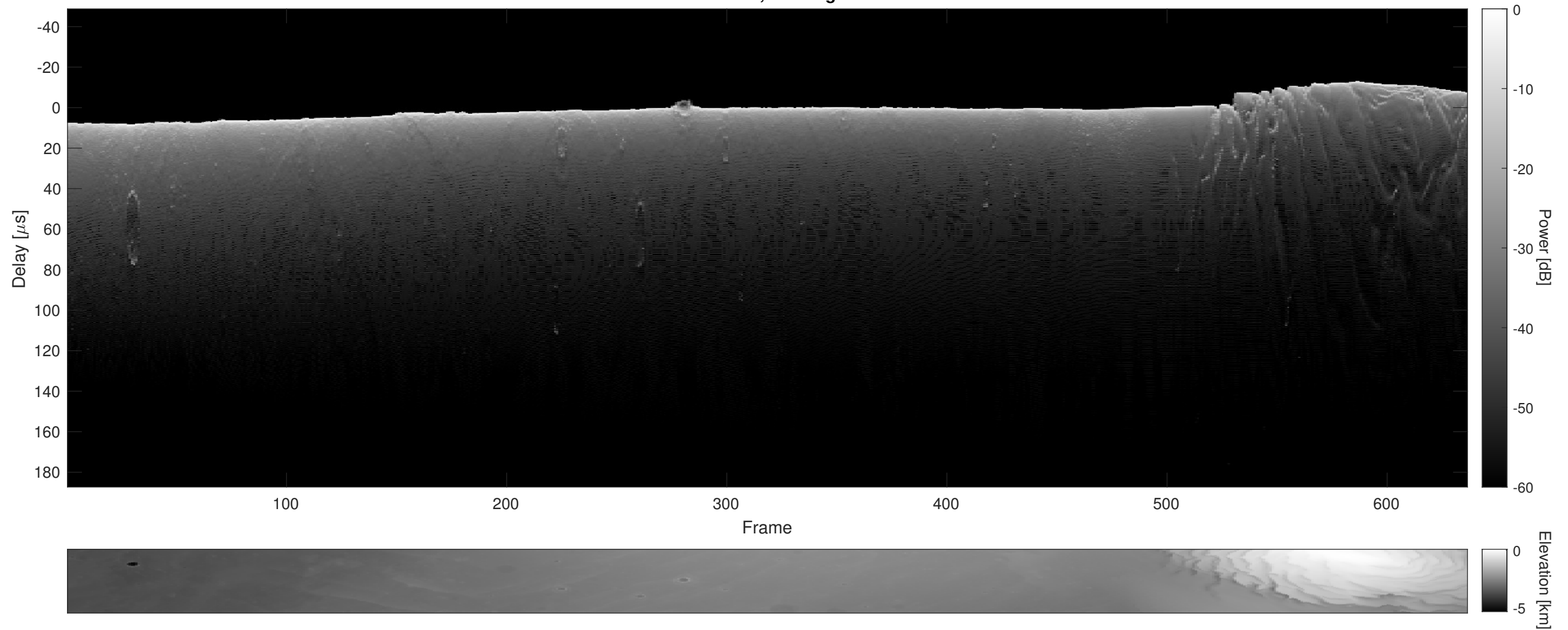
Orbit 22363, Cluttergram
