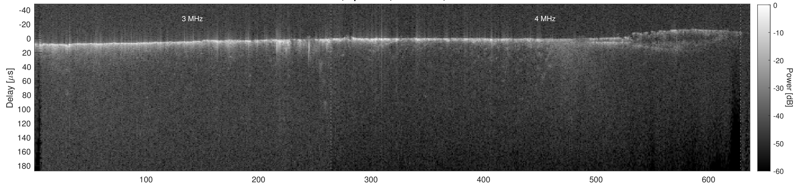
Orbit 22363, Cluttergram
