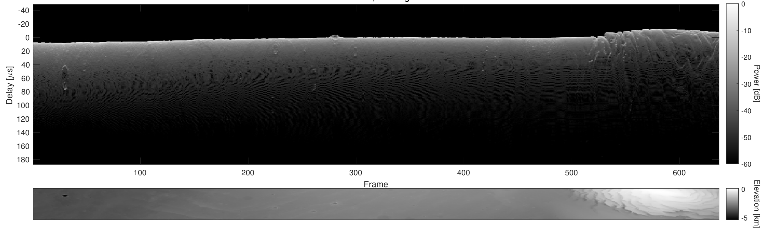
Orbit 22363, Cluttergram
