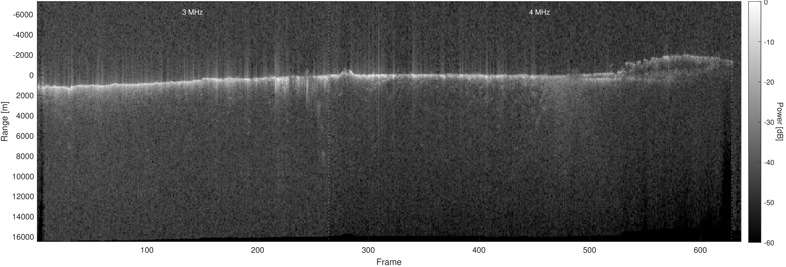
Orbit 22363, Optimized, No Window, Depth-Corrected, Channel 2
