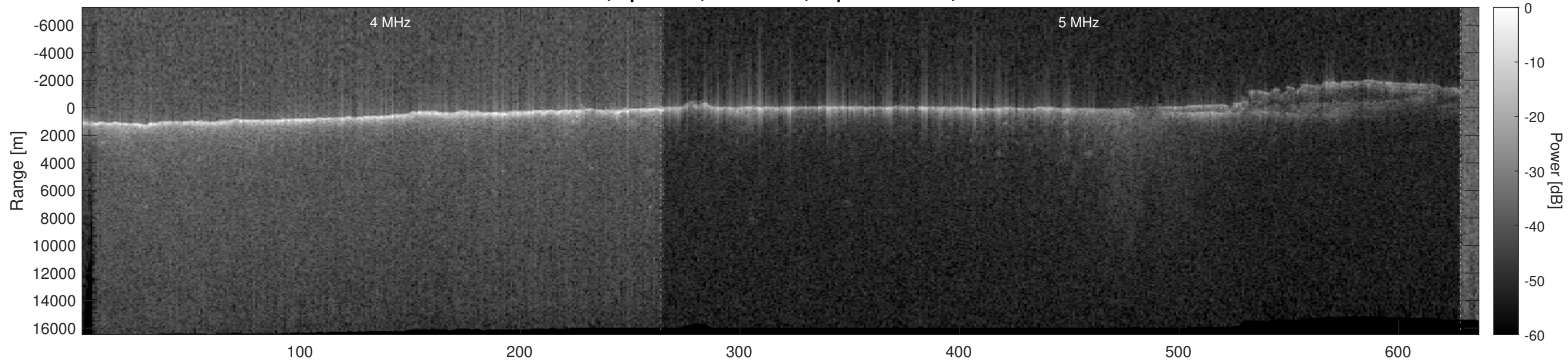
Orbit 22363, Optimized, No Window, Depth-Corrected, Channel 2
