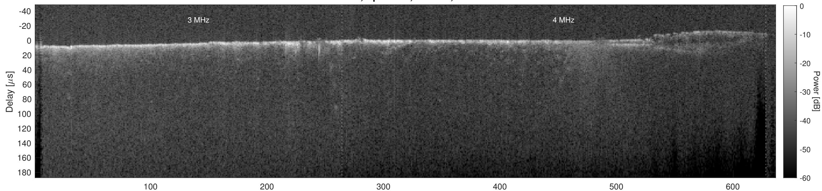
Orbit 22363, Cluttergram
