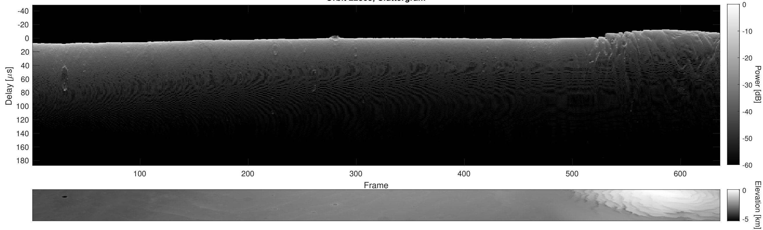
Orbit 22363, Cluttergram
