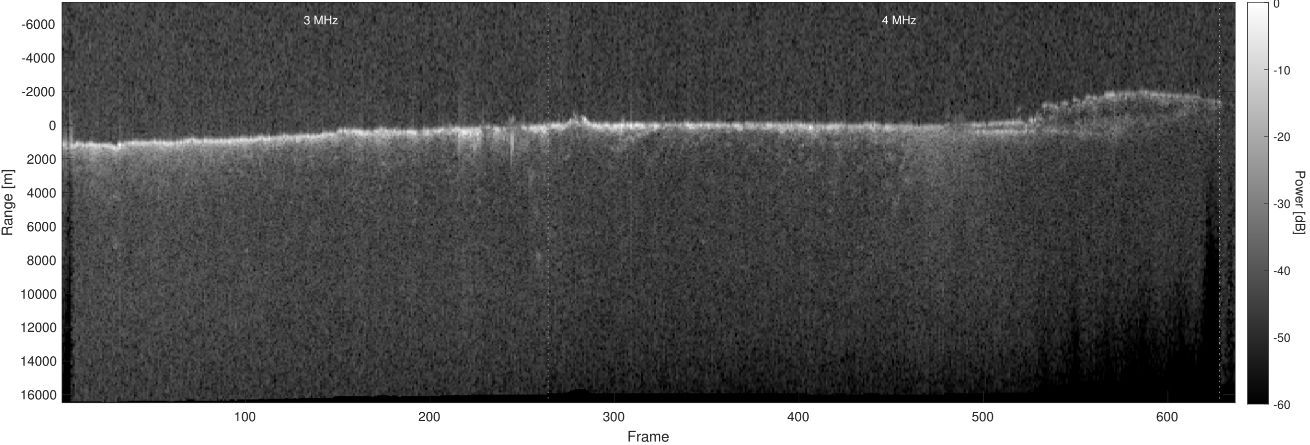
Orbit 22363, Optimized, Window, Depth-Corrected, Channel 2
