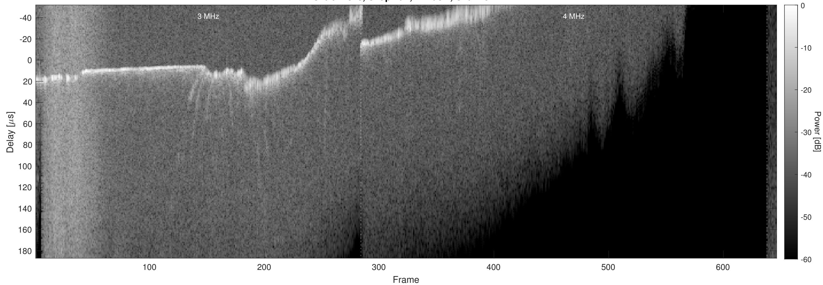
Orbit 22373, Chapman, Window, Channel 2
