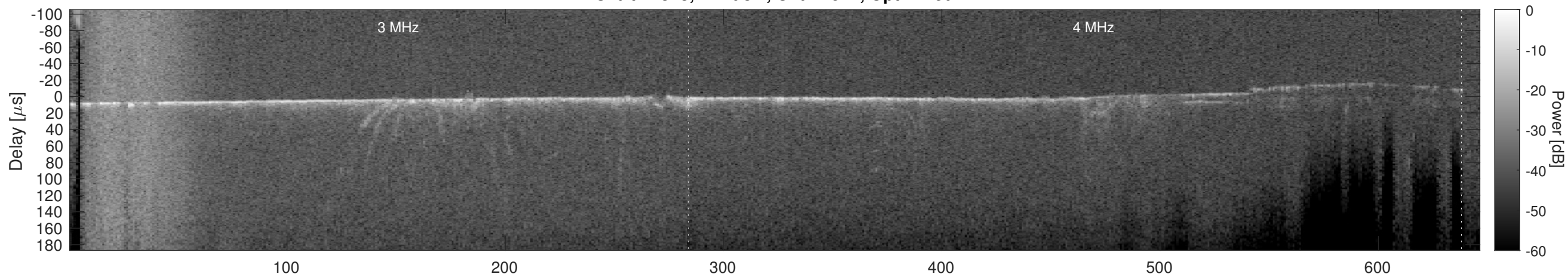
Orbit 22373, Cluttergram
