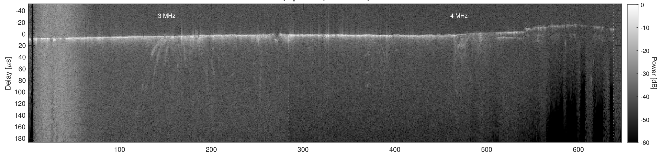
Orbit 22373, Cluttergram
